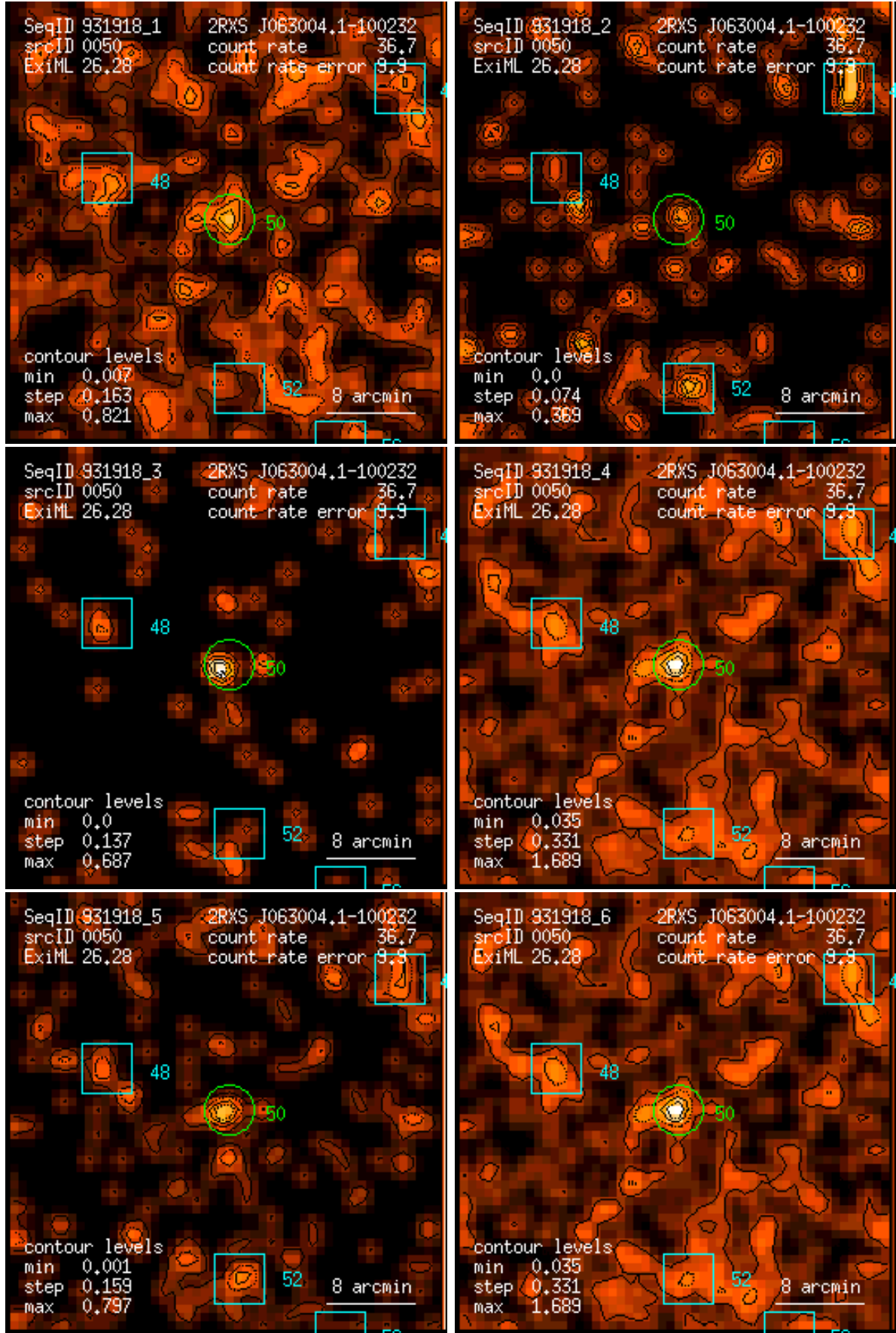
Figure 50: RASS 931918: detection 0050: band rate images, Gaussian filter: (1) PSPC channels 11 – 41, (2) 52 – 90, (3) 91 – 201, (4) 11 – 235, (5) 52 – 201, (6) 11 – 201. Broad band rates in counts/ks. Band rate contour levels in counts/ks/arcmin 2 .
