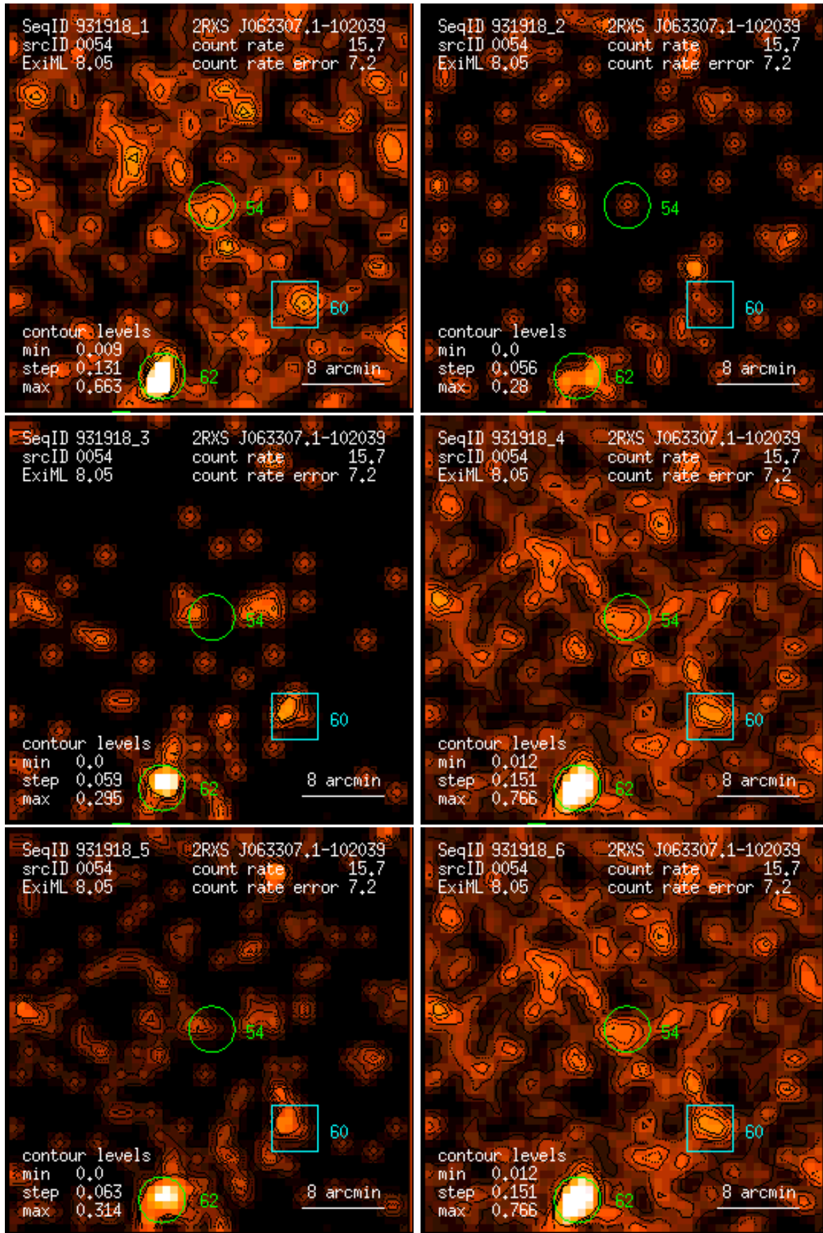
Figure 54: RASS 931918: detection 0054: band rate images, Gaussian filter: (1) PSPC channels 11 – 41, (2) 52 – 90, (3) 91 – 201, (4) 11 – 235, (5) 52 – 201, (6) 11 – 201. Broad band rates in counts/ks. Band rate contour levels in counts/ks/arcmin 2 .
