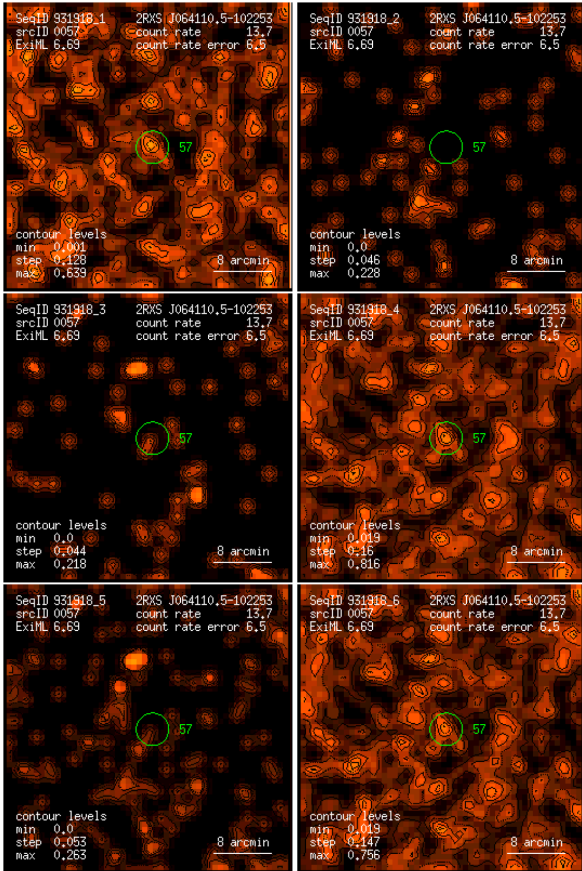
Figure 57: RASS 931918: detection 0057: band rate images, Gaussian filter: (1) PSPC channels 11 – 41, (2) 52 – 90, (3) 91 – 201, (4) 11 – 235, (5) 52 – 201, (6) 11 – 201. Broad band rates in counts/ks. Band rate contour levels in counts/ks/arcmin 2 .
