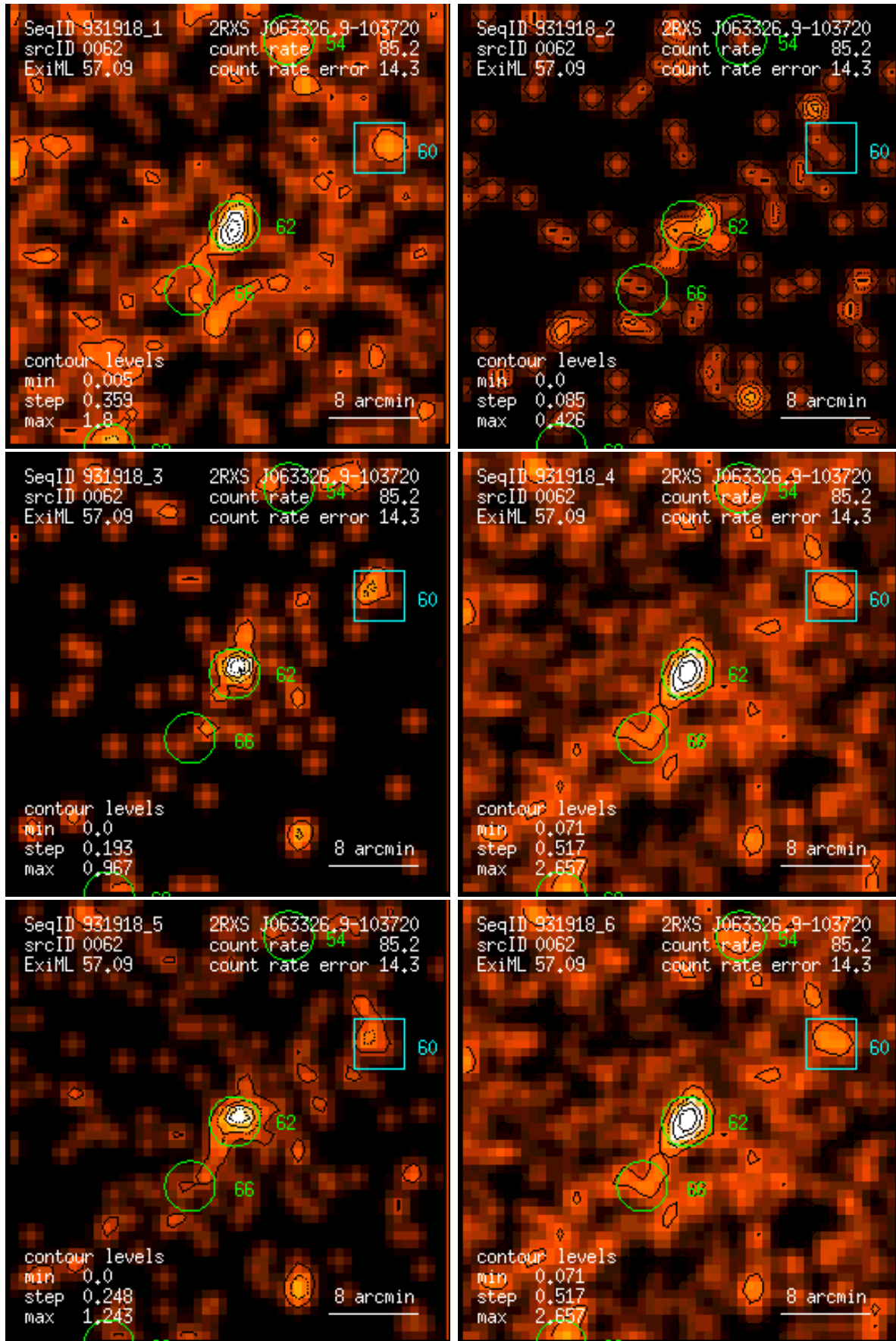
Figure 62: RASS 931918: detection 0062: band rate images, Gaussian filter: (1) PSPC channels 11 – 41, (2) 52 – 90, (3) 91 – 201, (4) 11 – 235, (5) 52 – 201, (6) 11 – 201. Broad band rates in counts/ks. Band rate contour levels in counts/ks/arcmin 2 .
