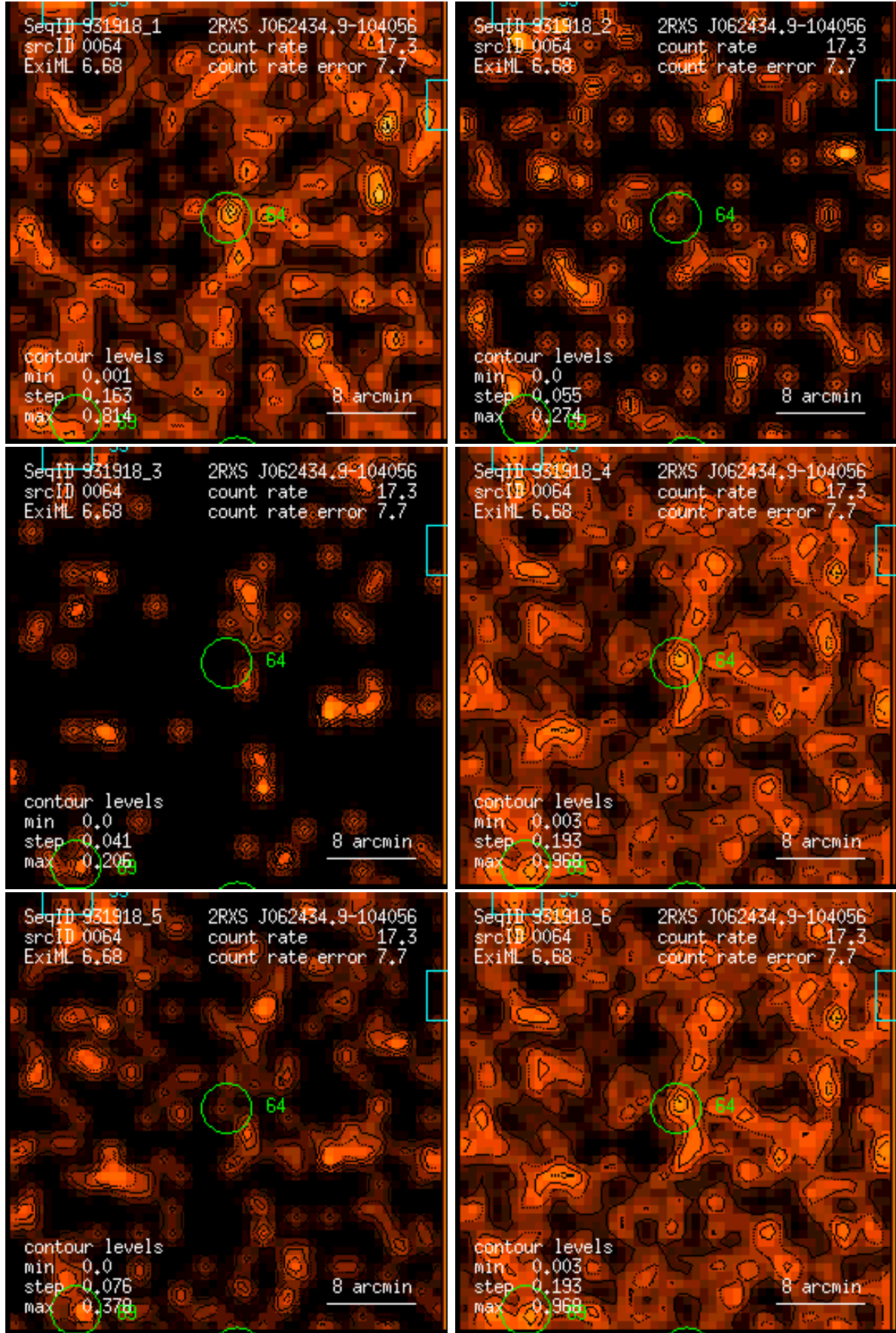
Figure 64: RASS 931918: detection 0064: band rate images, Gaussian filter: (1) PSPC channels 11 – 41, (2) 52 – 90, (3) 91 – 201, (4) 11 – 235, (5) 52 – 201, (6) 11 – 201. Broad band rates in counts/ks. Band rate contour levels in counts/ks/arcmin 2 .
