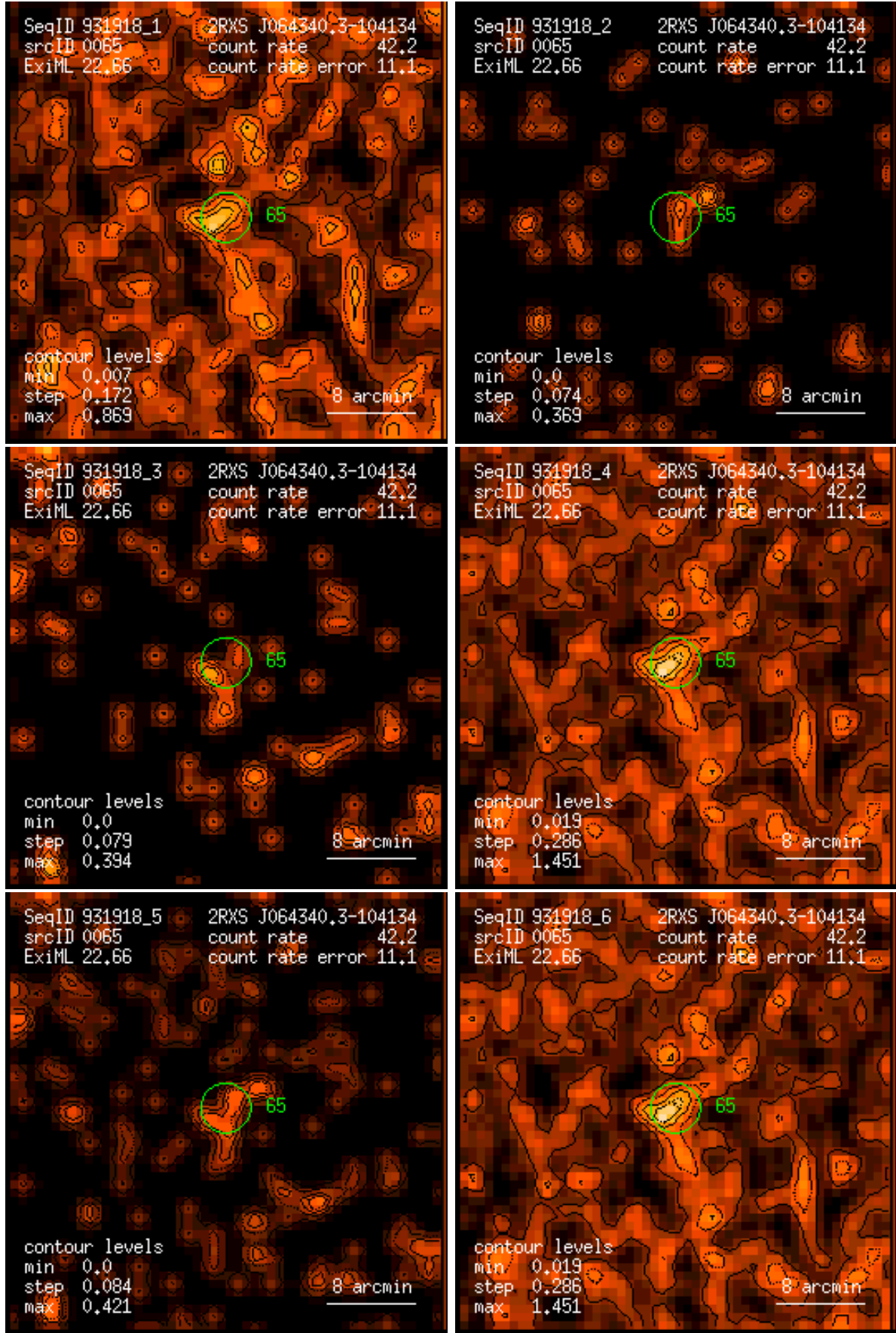
Figure 65: RASS 931918: detection 0065: band rate images, Gaussian filter: (1) PSPC channels 11 – 41, (2) 52 – 90, (3) 91 – 201, (4) 11 – 235, (5) 52 – 201, (6) 11 – 201. Broad band rates in counts/ks. Band rate contour levels in counts/ks/arcmin 2 .
