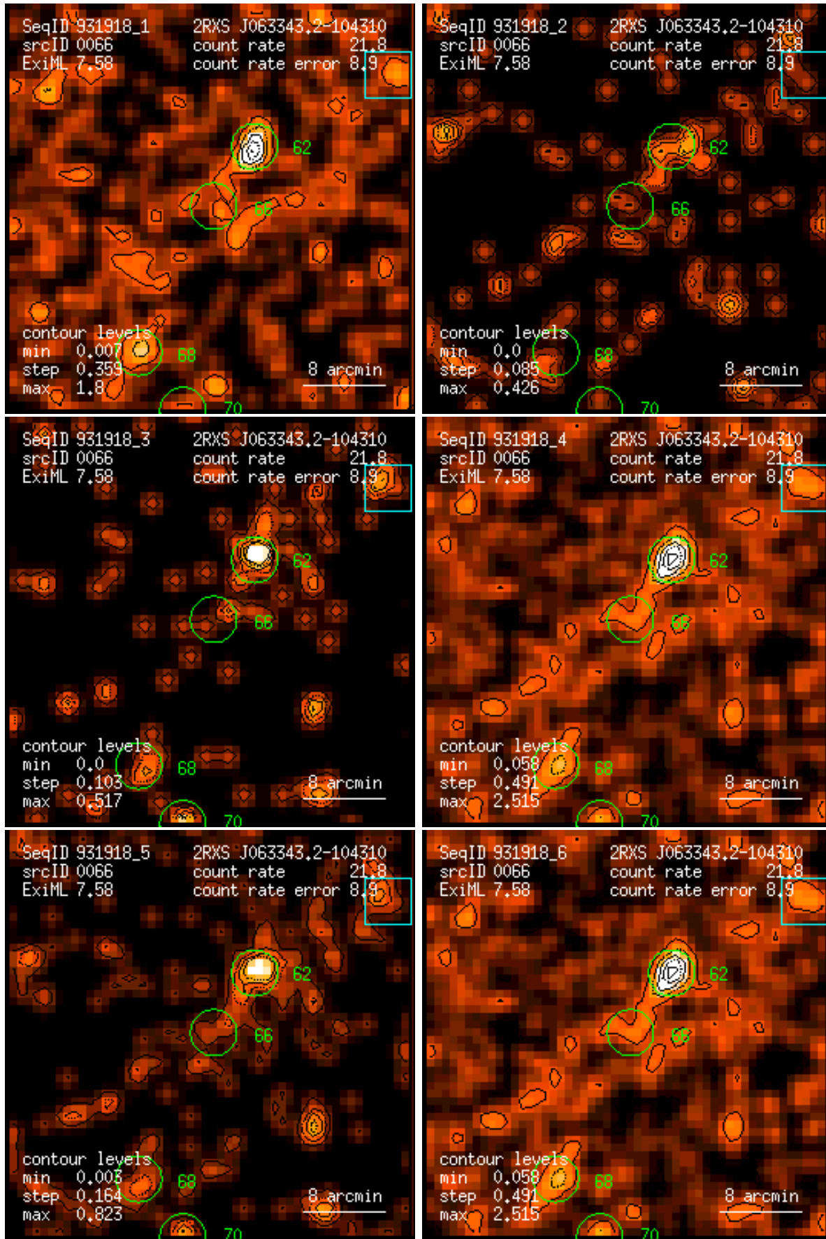
Figure 66: RASS 931918: detection 0066: band rate images, Gaussian filter: (1) PSPC channels 11 – 41, (2) 52 – 90, (3) 91 – 201, (4) 11 – 235, (5) 52 – 201, (6) 11 – 201. Broad band rates in counts/ks. Band rate contour levels in counts/ks/arcmin 2 .
