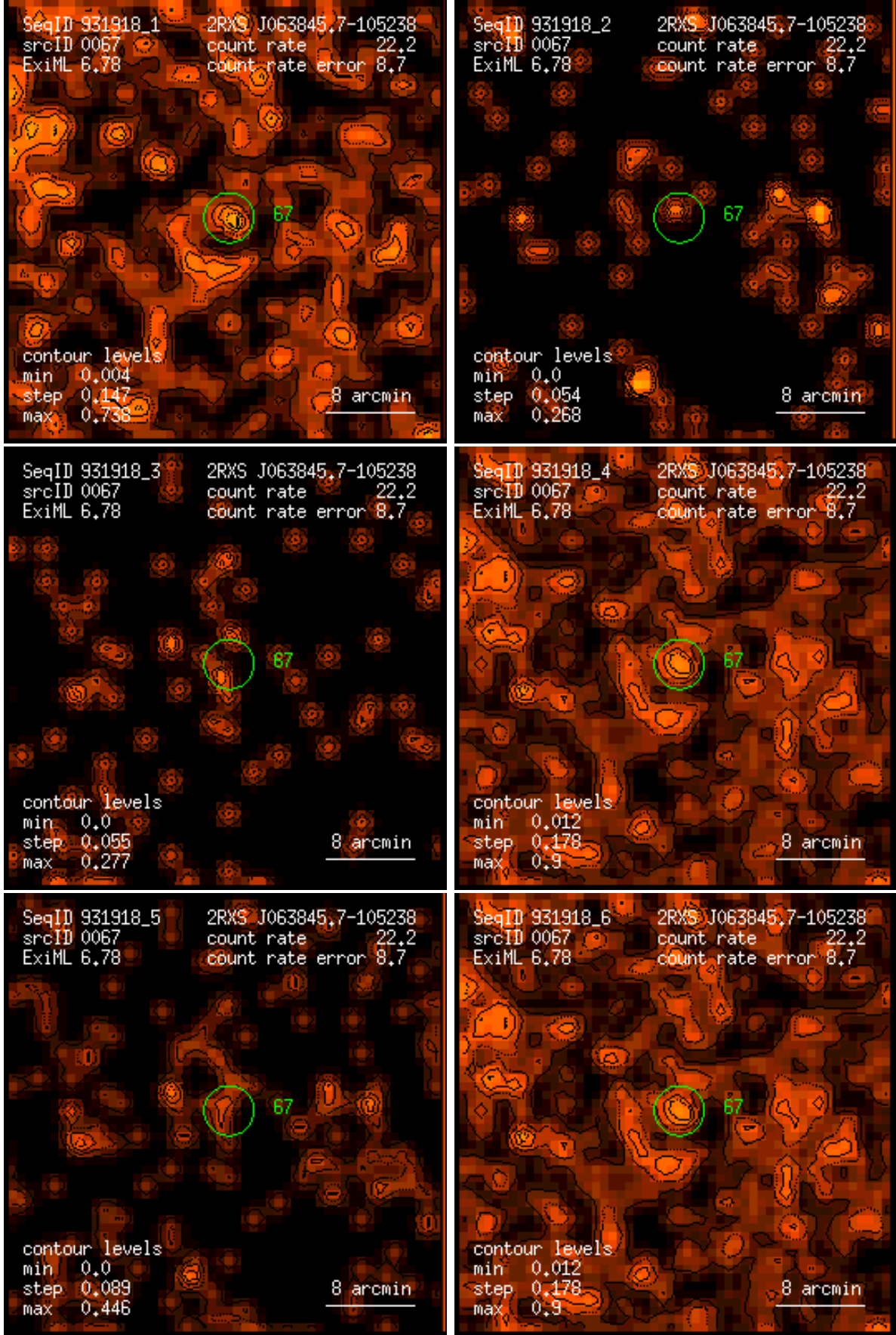
Figure 67: RASS 931918: detection 0067: band rate images, Gaussian filter: (1) PSPC channels 11 – 41, (2) 52 – 90, (3) 91 – 201, (4) 11 – 235, (5) 52 – 201, (6) 11 – 201. Broad band rates in counts/ks. Band rate contour levels in counts/ks/arcmin 2 .
