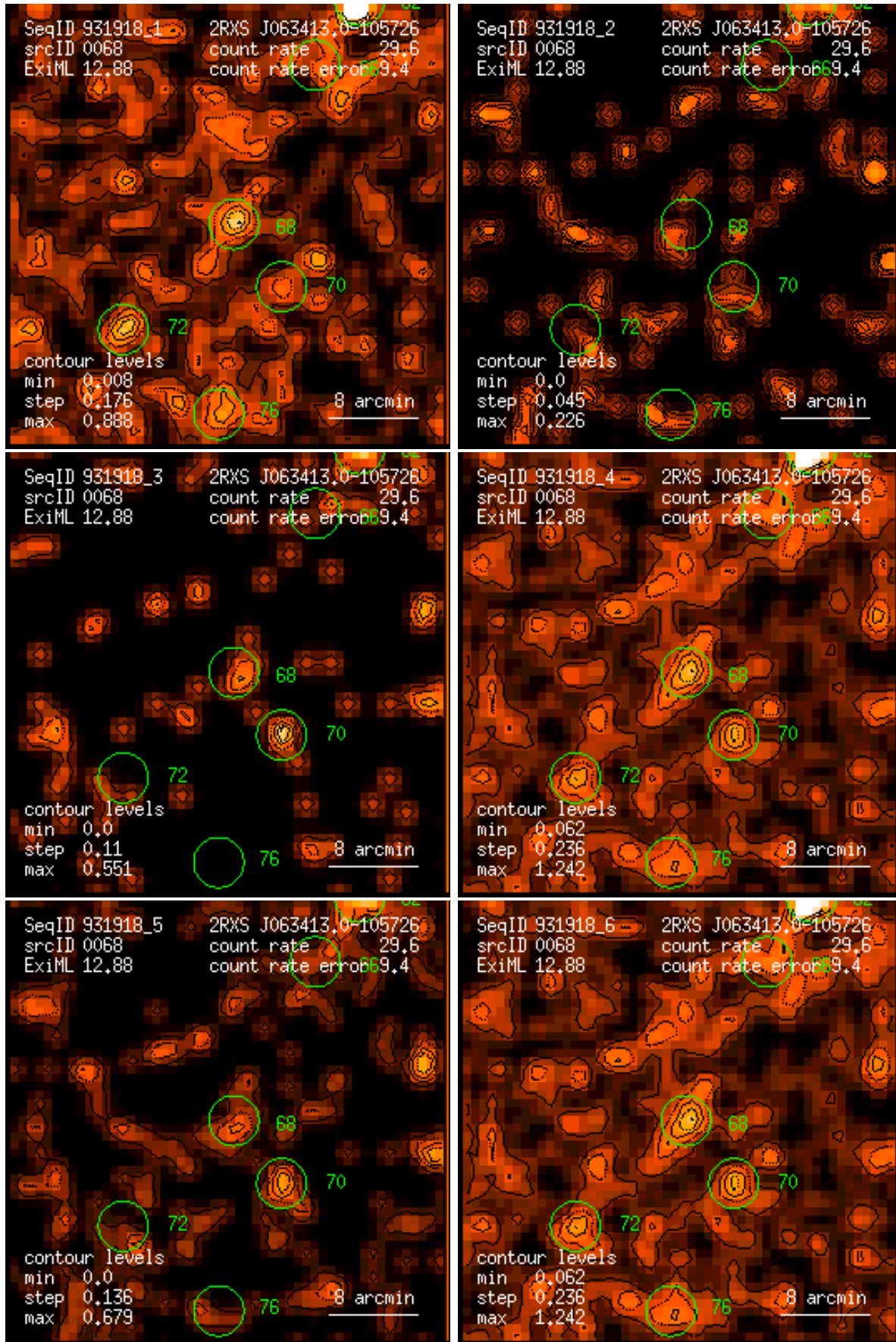
Figure 68: RASS 931918: detection 0068: band rate images, Gaussian filter: (1) PSPC channels 11 – 41, (2) 52 – 90, (3) 91 – 201, (4) 11 – 235, (5) 52 – 201, (6) 11 – 201. Broad band rates in counts/ks. Band rate contour levels in counts/ks/arcmin 2 .
