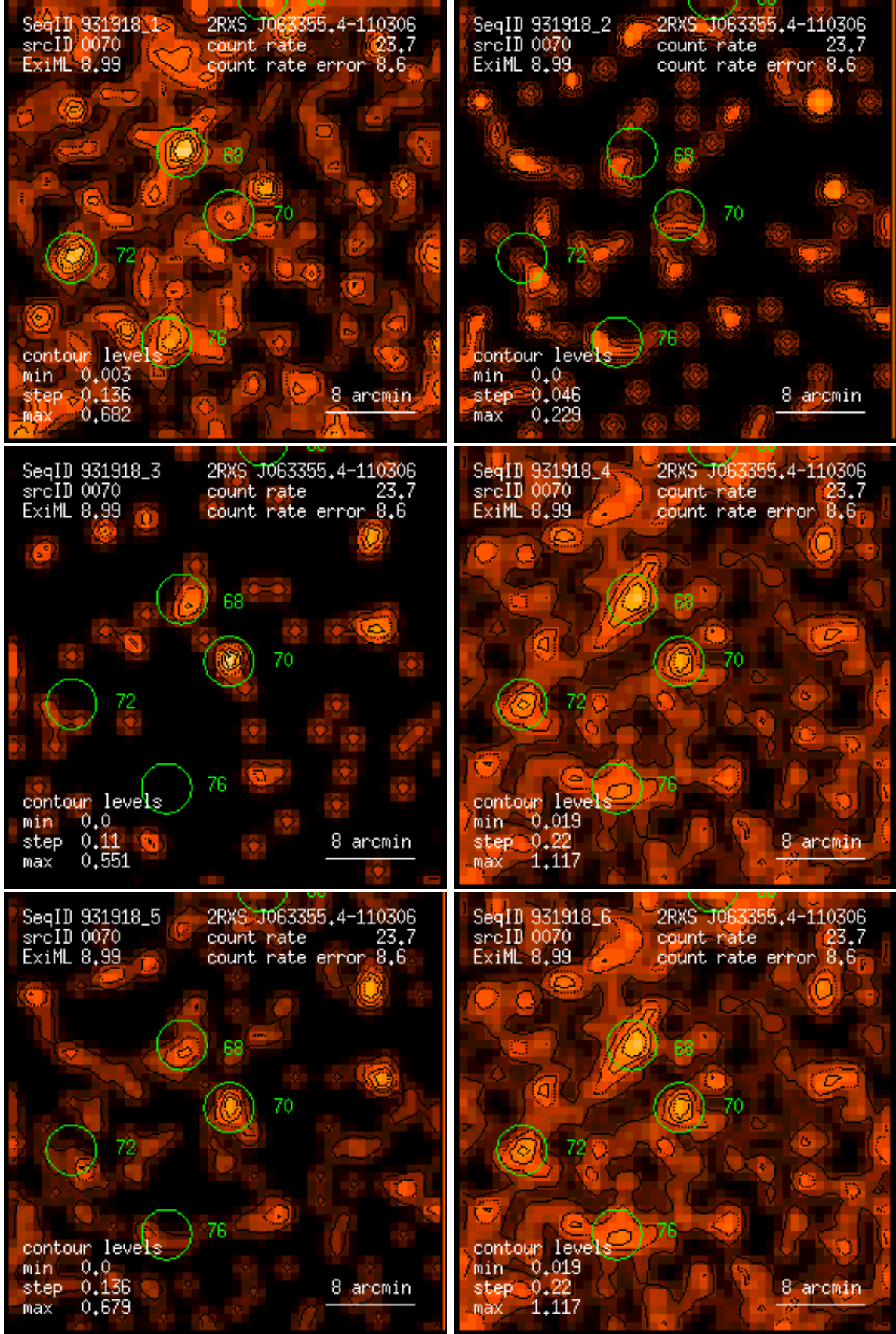
Figure 70: RASS 931918: detection 0070: band rate images, Gaussian filter: (1) PSPC channels 11 – 41, (2) 52 – 90, (3) 91 – 201, (4) 11 – 235, (5) 52 – 201, (6) 11 – 201. Broad band rates in counts/ks. Band rate contour levels in counts/ks/arcmin 2 .
