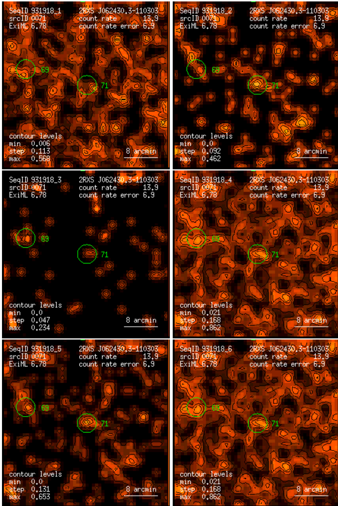
Figure 71: RASS 931918: detection 0071: band rate images, Gaussian filter: (1) PSPP channels 11 – 41, (2) 52 – 90, (3) 91 – 201, (4) 11 – 235, (5) 52 – 201, (6) 11 – 201. Broad band rates in counts/ks. Band rate contour levels in counts/ks/arcmin 2 .
