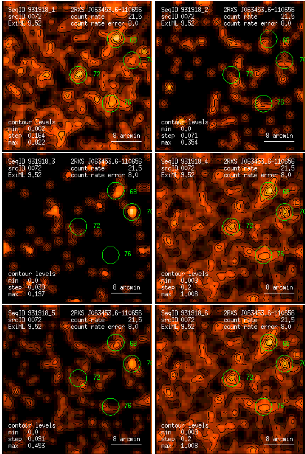
Figure 72: RASS 931918: detection 0072: band rate images, Gaussian filter: (1) PSPC channels 11 – 41, (2) 52 – 90, (3) 91 – 201, (4) 11 – 235, (5) 52 – 201, (6) 11 – 201. Broad band rates in counts/ks. Band rate contour levels in counts/ks/arcmin 2 .
