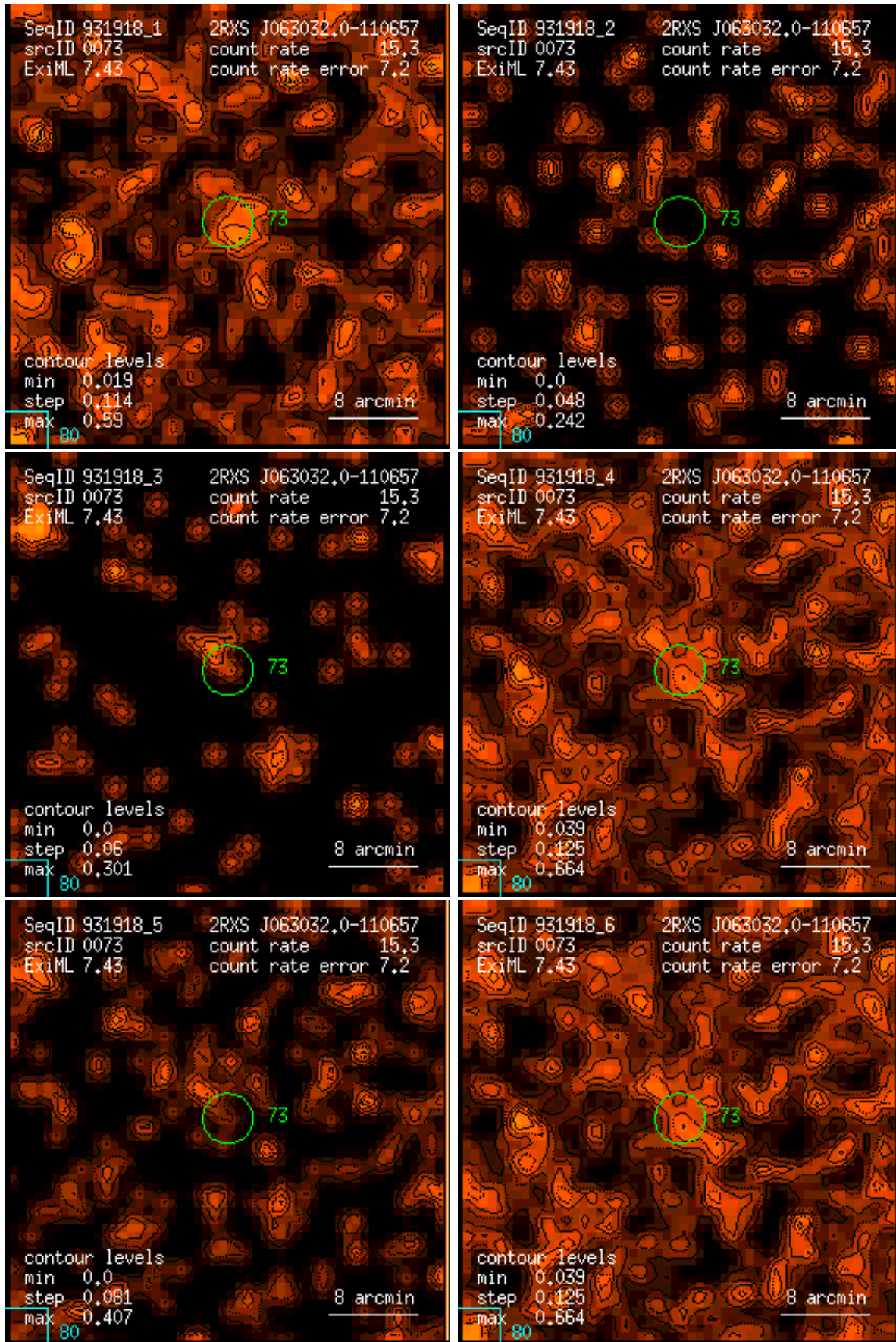
Figure 73: RASS 931918: detection 0073: band rate images, Gaussian filter: (1) PSPC channels 11 – 41, (2) 52 – 90, (3) 91 – 201, (4) 11 – 235, (5) 52 – 201, (6) 11 – 201. Broad band rates in counts/ks. Band rate contour levels in counts/ks/arcmin 2 .
