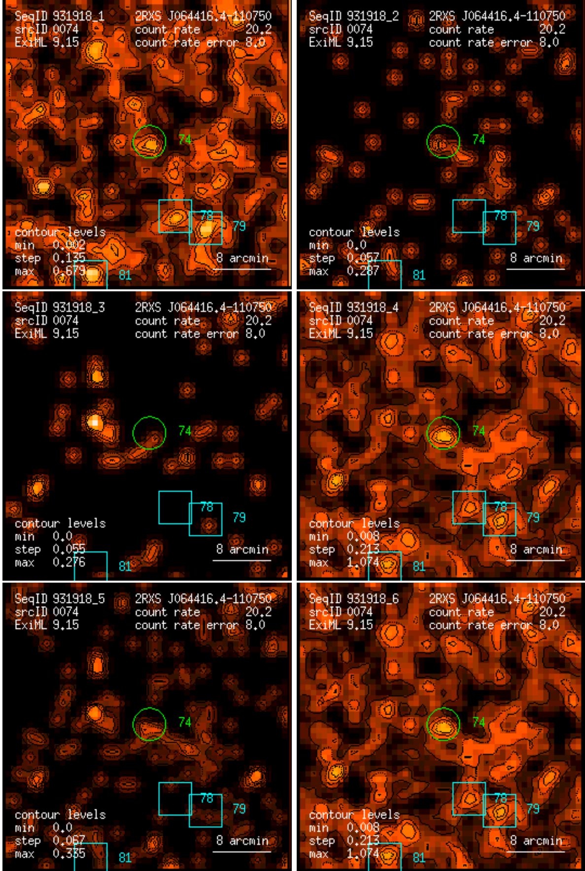
Figure 74: RASS 931918: detection 0074: band rate images, Gaussian filter: (1) PSPC channels 11 – 41, (2) 52 – 90, (3) 91 – 201, (4) 11 – 235, (5) 52 – 201, (6) 11 – 201. Broad band rates in counts/ks. Band rate contour levels in counts/ks/arcmin 2 .
