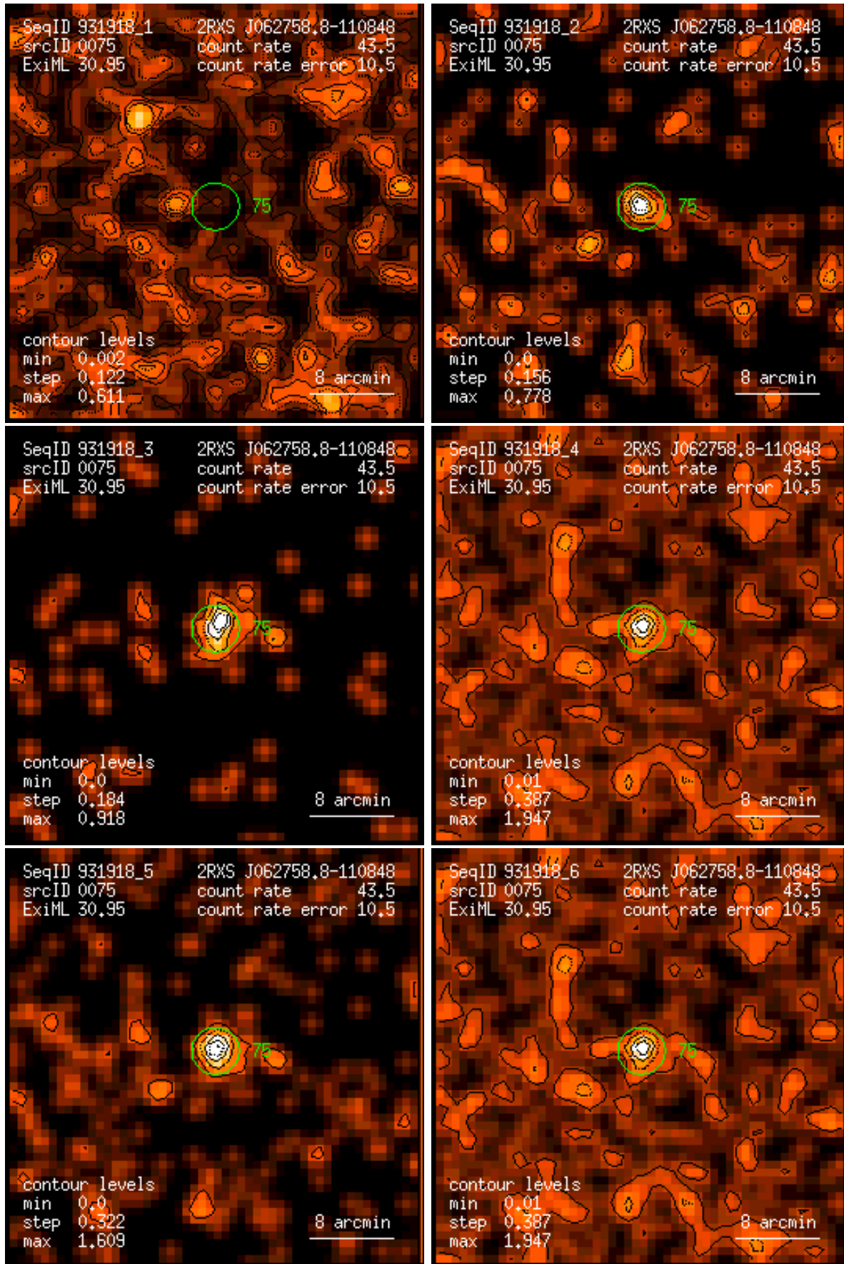
Figure 75: RASS 931918: detection 0075: band rate images, Gaussian filter: (1) PSPC channels 11 – 41, (2) 52 – 90, (3) 91 – 201, (4) 11 – 235, (5) 52 – 201, (6) 11 – 201. Broad band rates in counts/ks. Band rate contour levels in counts/ks/arcmin 2 .
