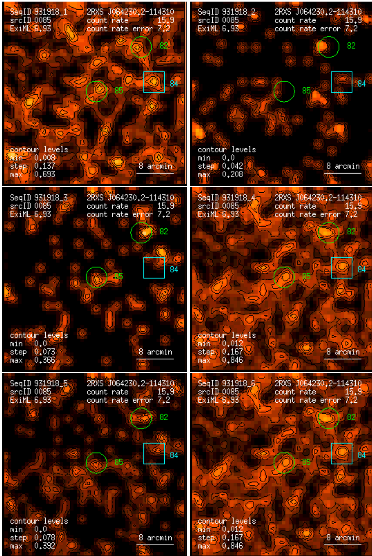
Figure 85: RASS 931918: detection 0085: band rate images, Gaussian filter: (1) PSPC channels 11 – 41, (2) 52 – 90, (3) 91 – 201, (4) 11 – 235, (5) 52 – 201, (6) 11 – 201. Broad band rates in counts/ks. Band rate contour levels in counts/ks/arcmin 2 .
