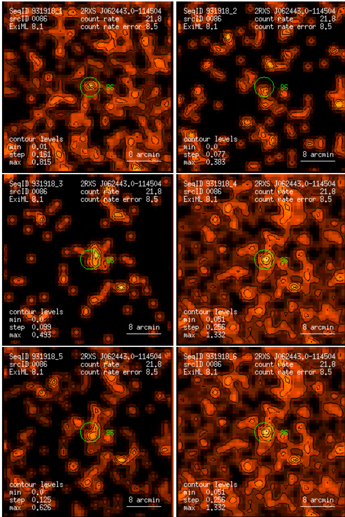
Figure 86: RASS 931918: detection 0086: band rate images, Gaussian filter: (1) PSPC channels 11 – 41, (2) 52 – 90, (3) 91 – 201, (4) 11 – 235, (5) 52 – 201, (6) 11 – 201. Broad band rates in counts/ks. Band rate contour levels in counts/ks/arcmin 2 .
