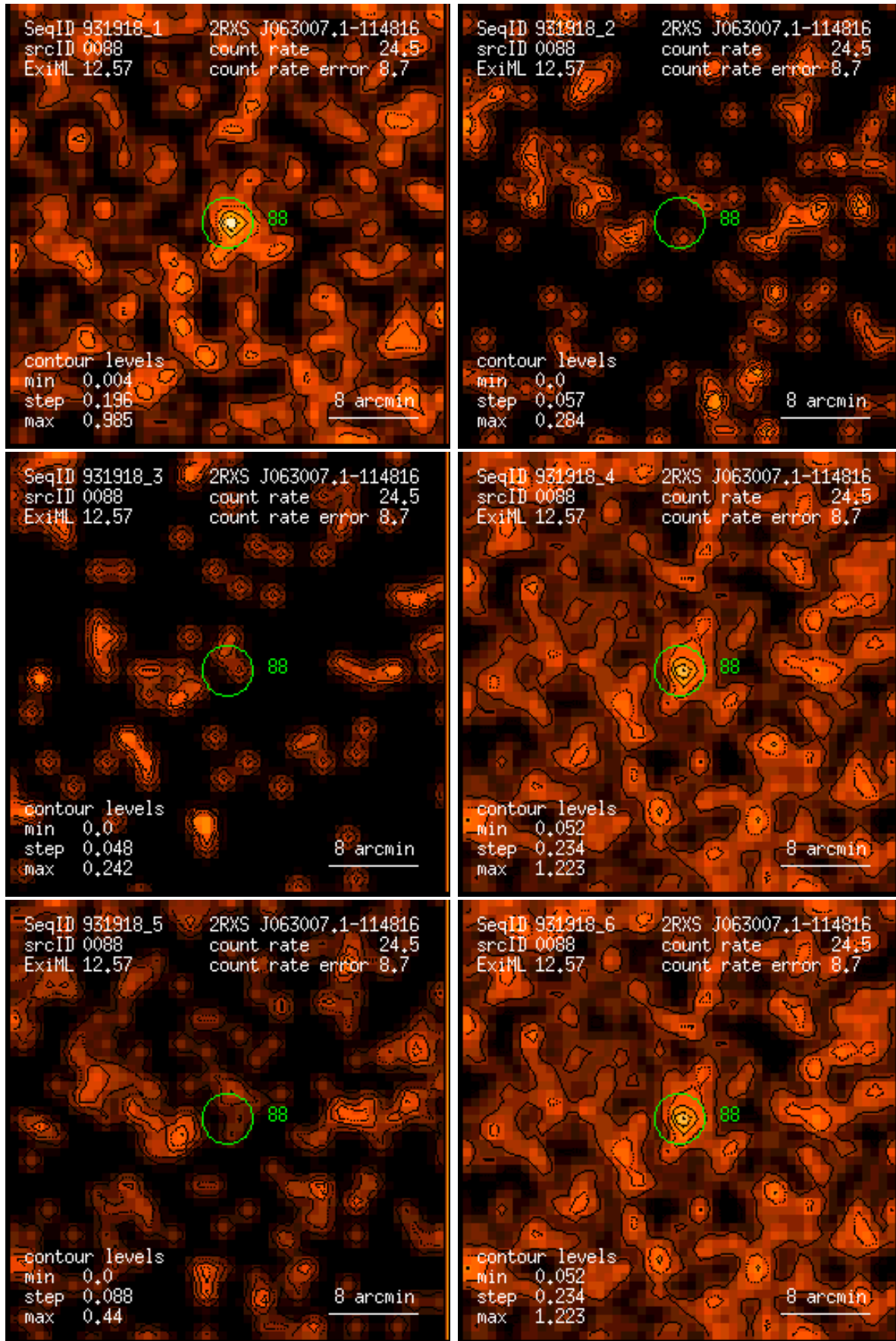
Figure 88: RASS 931918: detection 0088: band rate images, Gaussian filter: (1) PSPC channels 11 – 41, (2) 52 – 90, (3) 91 – 201, (4) 11 – 235, (5) 52 – 201, (6) 11 – 201. Broad band rates in counts/ks. Band rate contour levels in counts/ks/arcmin 2 .
