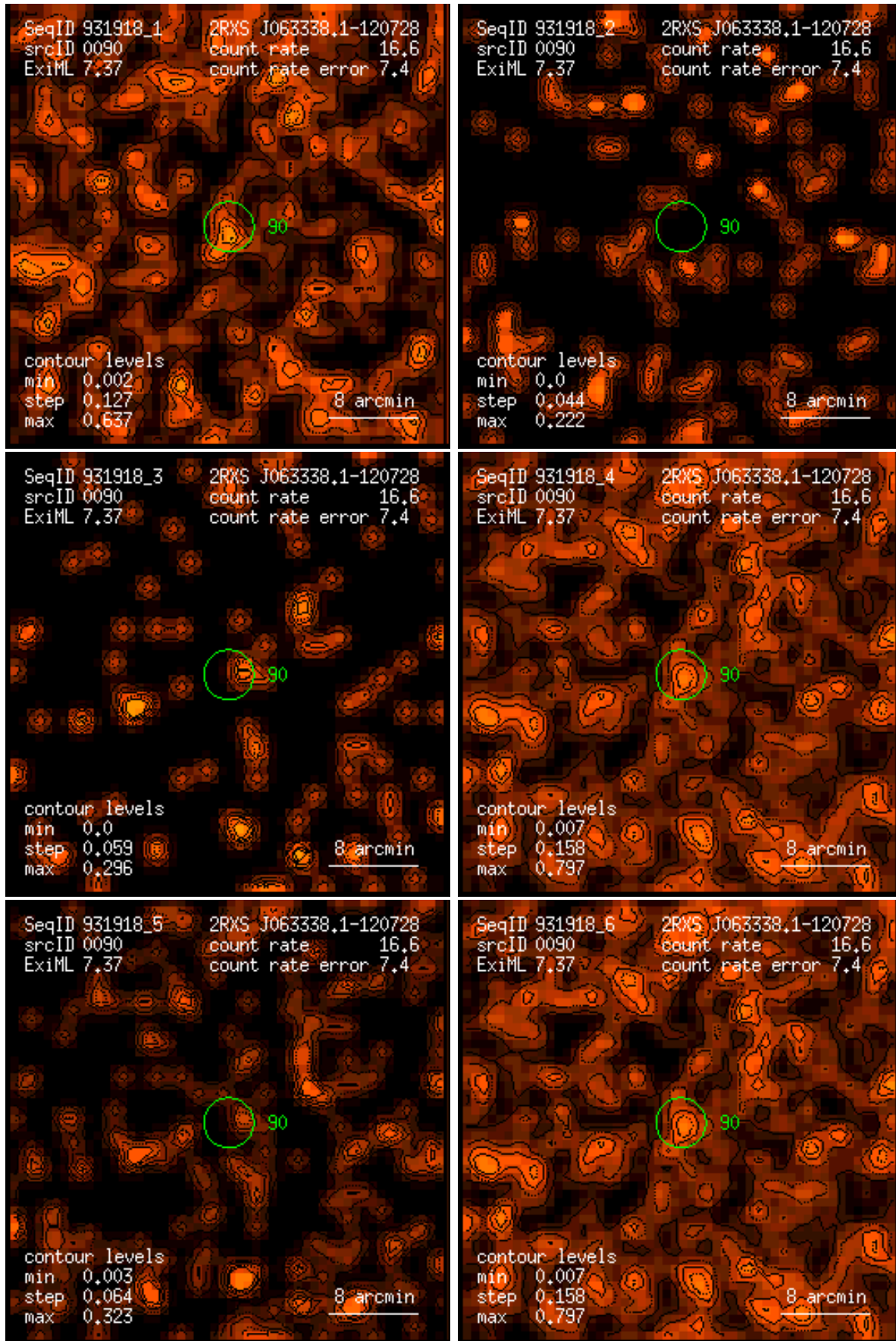
Figure 90: RASS 931918: detection 0090: band rate images, Gaussian filter: (1) PSPC channels 11 – 41, (2) 52 – 90, (3) 91 – 201, (4) 11 – 235, (5) 52 – 201, (6) 11 – 201. Broad band rates in counts/ks. Band rate contour levels in counts/ks/arcmin 2 .
