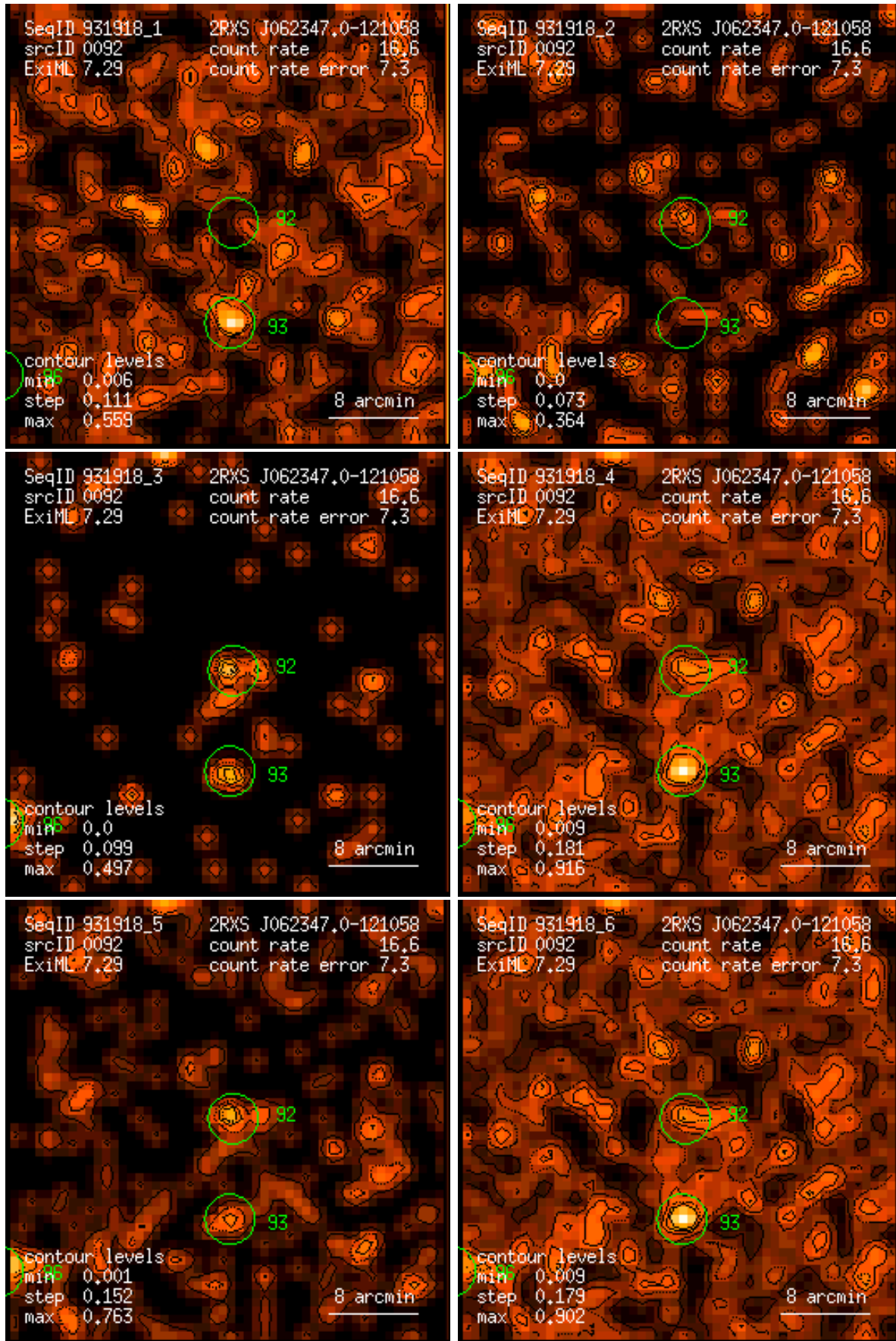
Figure 92: RASS 931918: detection 0092: band rate images, Gaussian filter: (1) PSPC channels 11 – 41, (2) 52 – 90, (3) 91 – 201, (4) 11 – 235, (5) 52 – 201, (6) 11 – 201. Broad band rates in counts/ks. Band rate contour levels in counts/ks/arcmin 2 .
