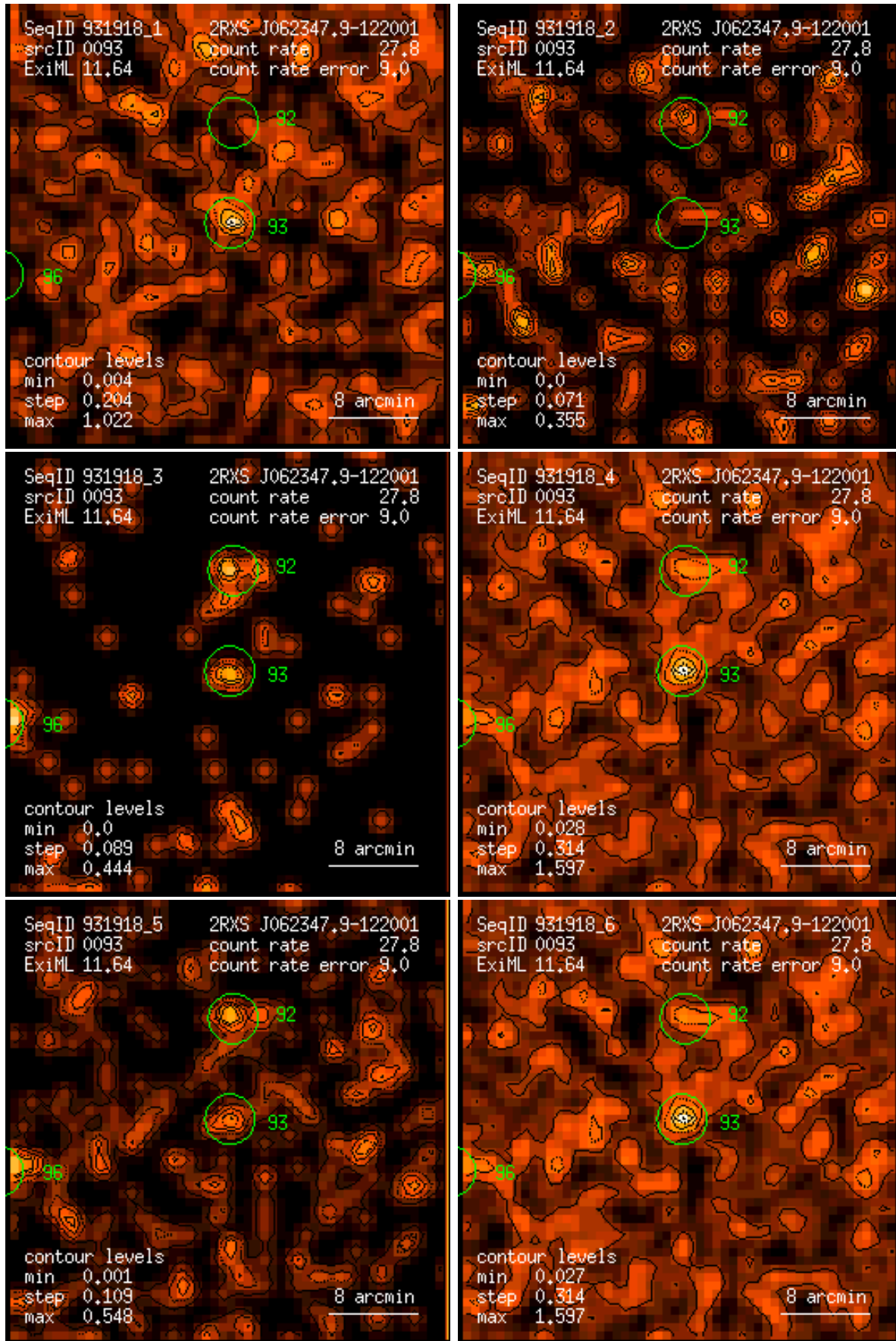
Figure 93: RASS 931918: detection 0093: band rate images, Gaussian filter: (1) PSPC channels 11 – 41, (2) 52 – 90, (3) 91 – 201, (4) 11 – 235, (5) 52 – 201, (6) 11 – 201. Broad band rates in counts/ks. Band rate contour levels in counts/ks/arcmin 2 .
