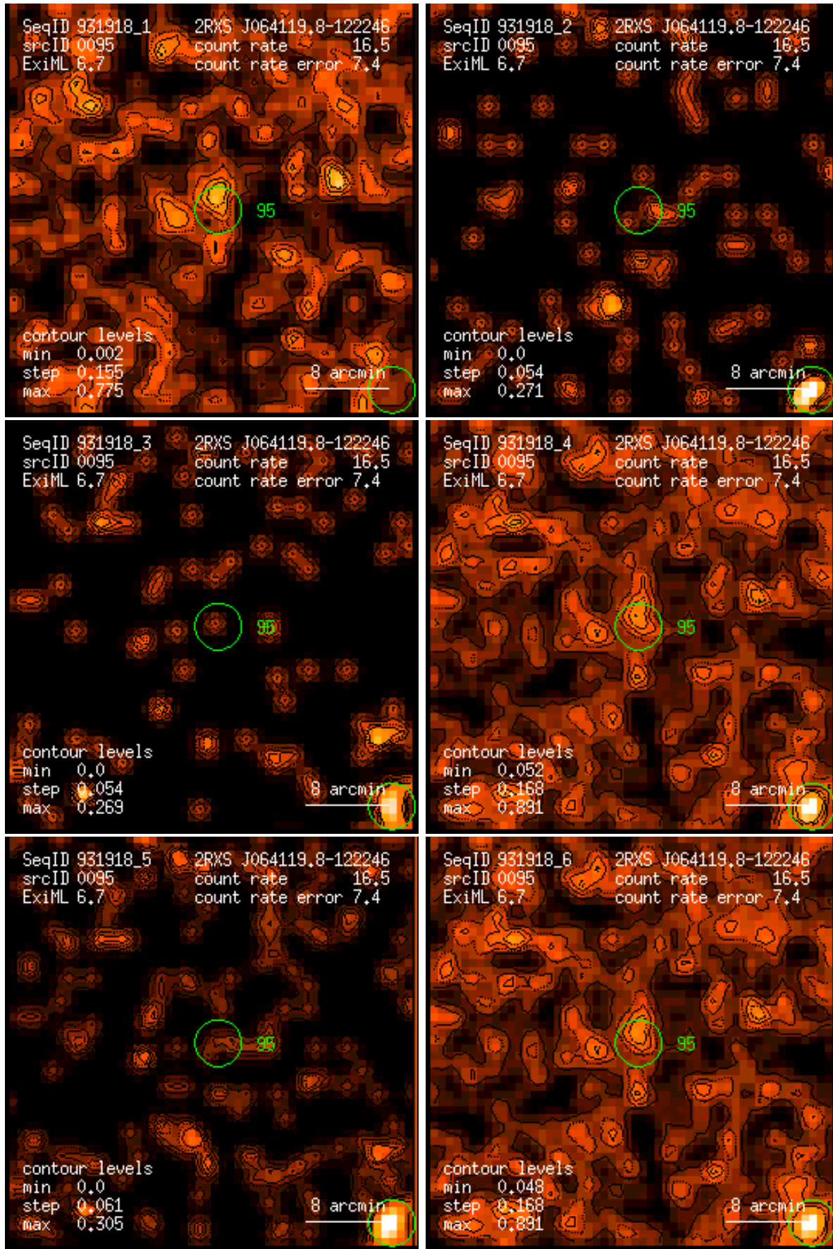
Figure 95: RASS 931918: detection 0095: band rate images, Gaussian filter: (1) PSPC channels 11 – 41, (2) 52 – 90, (3) 91 – 201, (4) 11 – 235, (5) 52 – 201, (6) 11 – 201. Broad band rates in counts/ks. Band rate contour levels in counts/ks/arcmin 2 .
