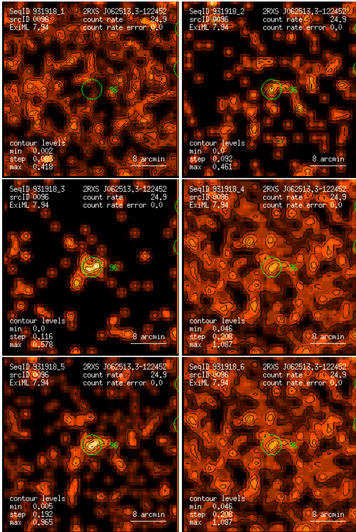
Figure 96: RASS 931918: detection 0096: band rate images, Gaussian filter: (1) PSPC channels 11 – 41, (2) 52 – 90, (3) 91 – 201, (4) 11 – 235, (5) 52 – 201, (6) 11 – 201. Broad band rates in counts/ks. Band rate contour levels in counts/ks/arcmin 2 .
