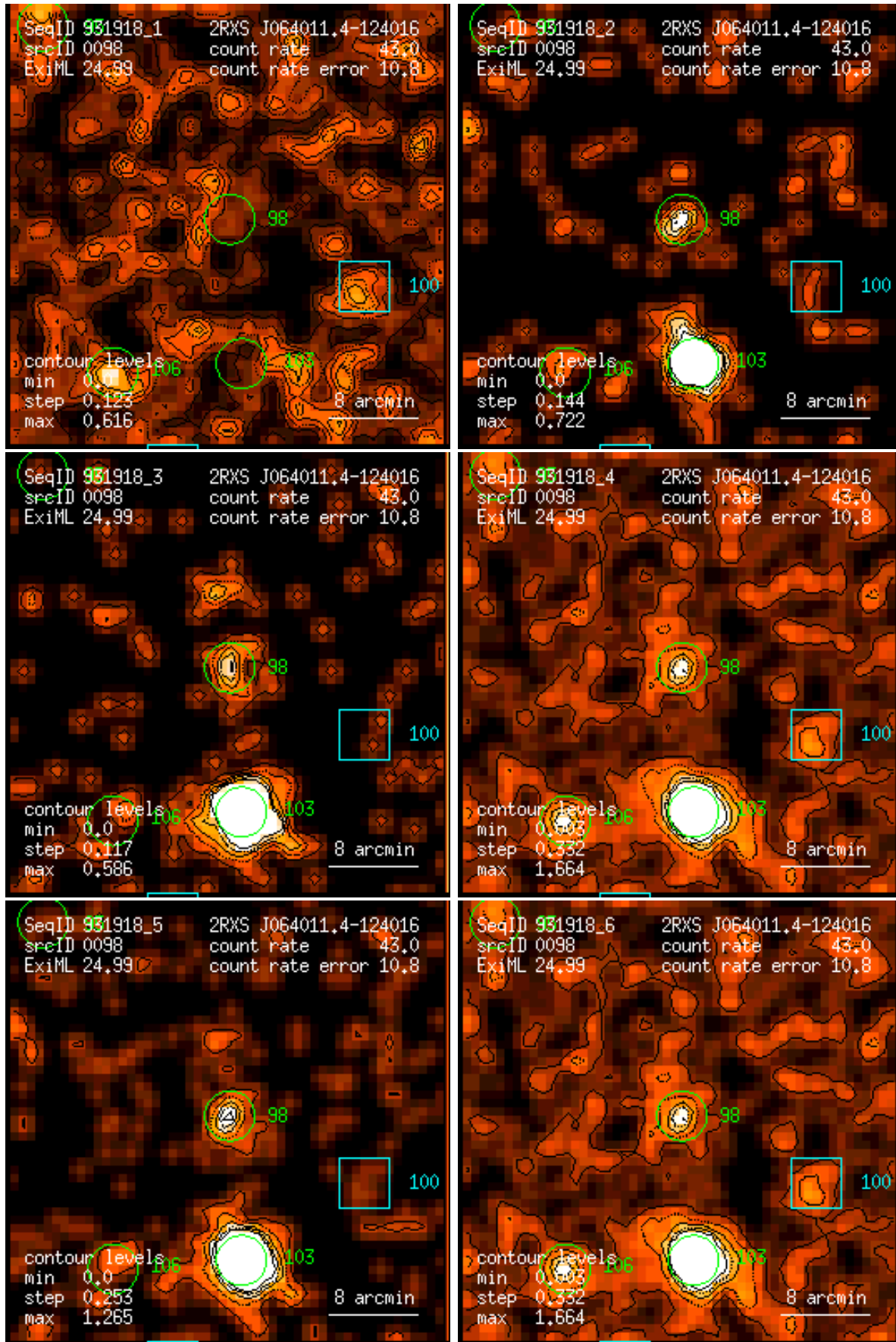
Figure 98: RASS 931918: detection 0098: band rate images, Gaussian filter: (1) PSPC channels 11 – 41, (2) 52 – 90, (3) 91 – 201, (4) 11 – 235, (5) 52 – 201, (6) 11 – 201. Broad band rates in counts/ks. Band rate contour levels in counts/ks/arcmin 2 .
