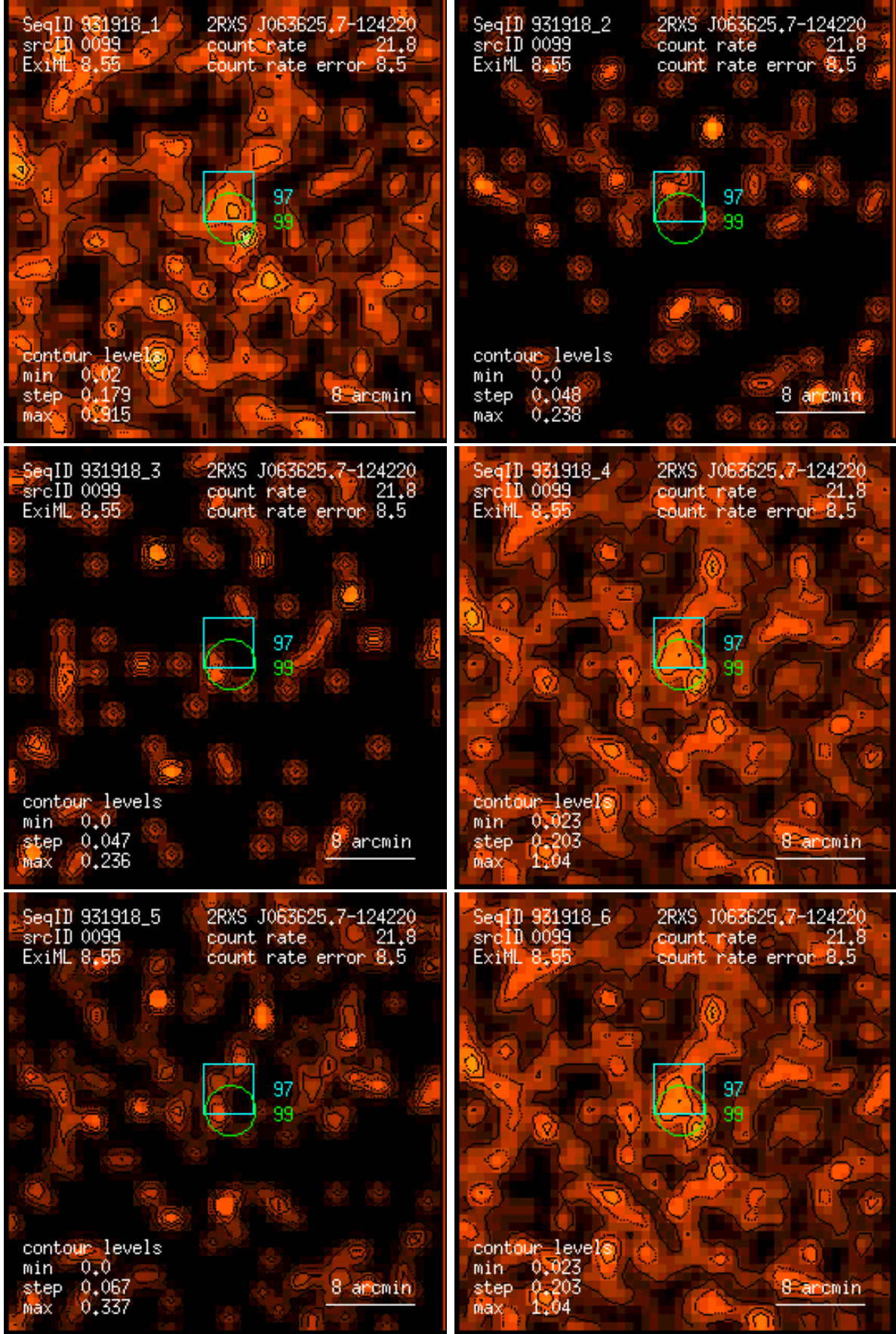
Figure 99: RASS 931918: detection 0099: band rate images, Gaussian filter: (1) PSPC channels 11 – 41, (2) 52 – 90, (3) 91 – 201, (4) 11 – 235, (5) 52 – 201, (6) 11 – 201. Broad band rates in counts/ks. Band rate contour levels in counts/ks/arcmin 2 .
