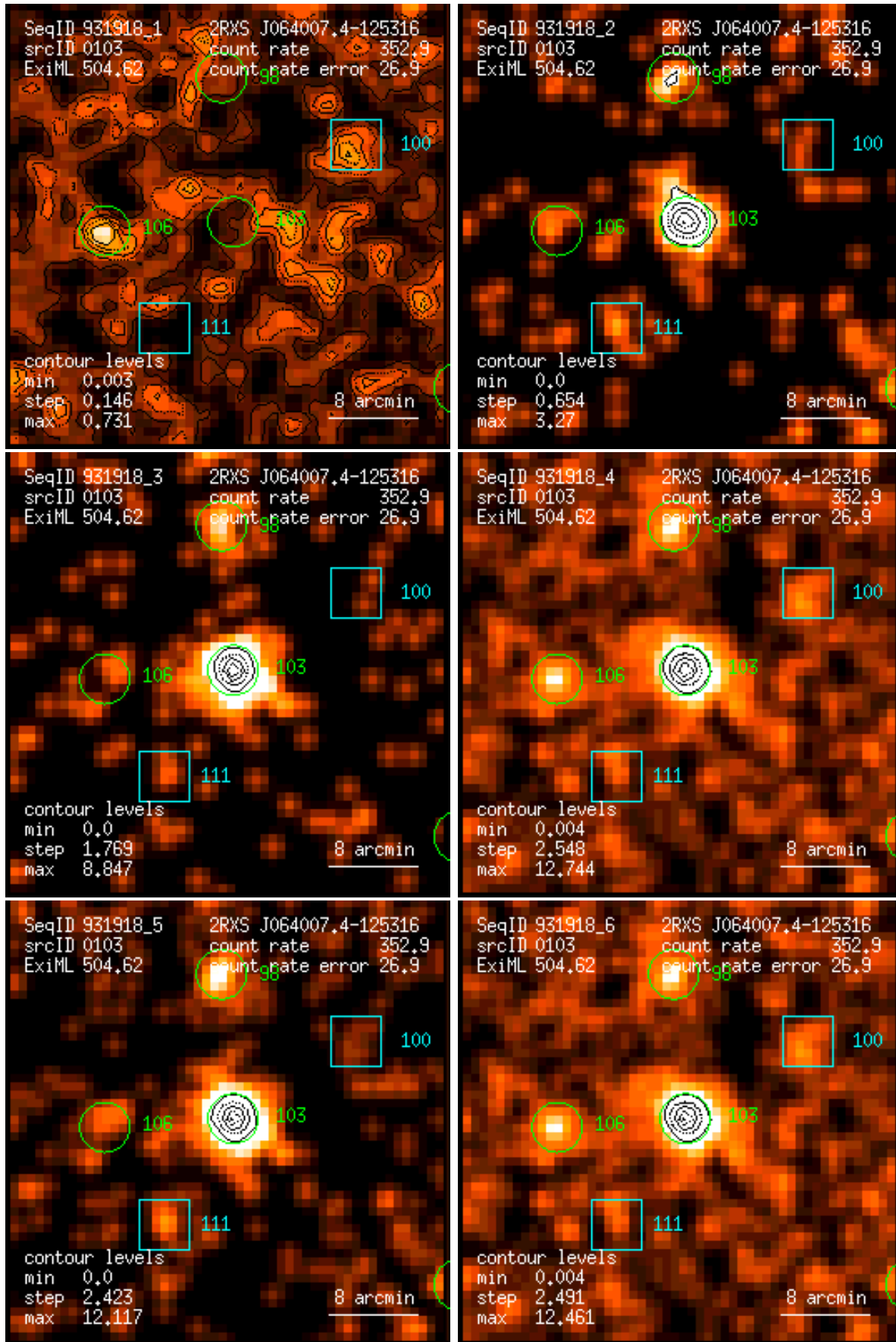
Figure 103: RASS 931918: detection 0103: band rate images, Gaussian filter: (1) PSPC channels 11 – 41, (2) 52 – 90, (3) 91 – 201, (4) 11 – 235, (5) 52 – 201, (6) 11 – 201. Broad band rates in counts/ks. Band rate contour levels in counts/ks/arcmin 2 .
