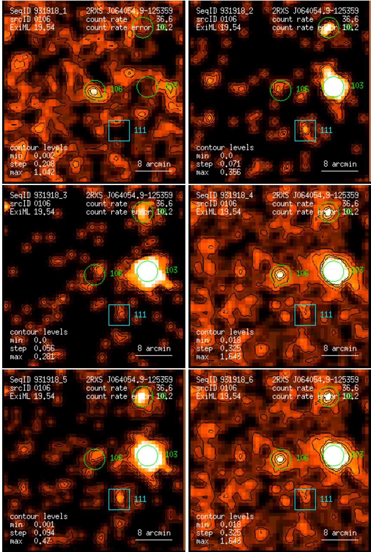
Figure 106: RASS 931918: detection 0106: band rate images, Gaussian filter: (1) PSPC channels 11 – 41, (2) 52 – 90, (3) 91 – 201, (4) 11 – 235, (5) 52 – 201, (6) 11 – 201. Broad band rates in counts/ks. Band rate contour levels in counts/ks/arcmin 2 .
