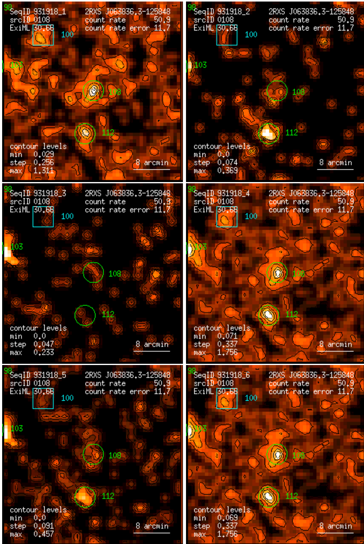
Figure 108: RASS 931918: detection 0108: band rate images, Gaussian filter: (1) PSPC channels 11 – 41, (2) 52 – 90, (3) 91 – 201, (4) 11 – 235, (5) 52 – 201, (6) 11 – 201. Broad band rates in counts/ks. Band rate contour levels in counts/ks/arcmin 2 .
