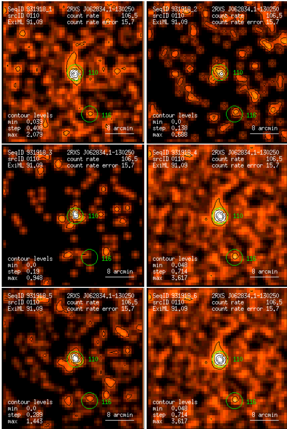
Figure 110: RASS 931918: detection 0110: band rate images, Gaussian filter: (1) PSPC channels 11 – 41, (2) 52 – 90, (3) 91 – 201, (4) 11 – 235, (5) 52 – 201, (6) 11 – 201. Broad band rates in counts/ks. Band rate contour levels in counts/ks/arcmin 2 .
