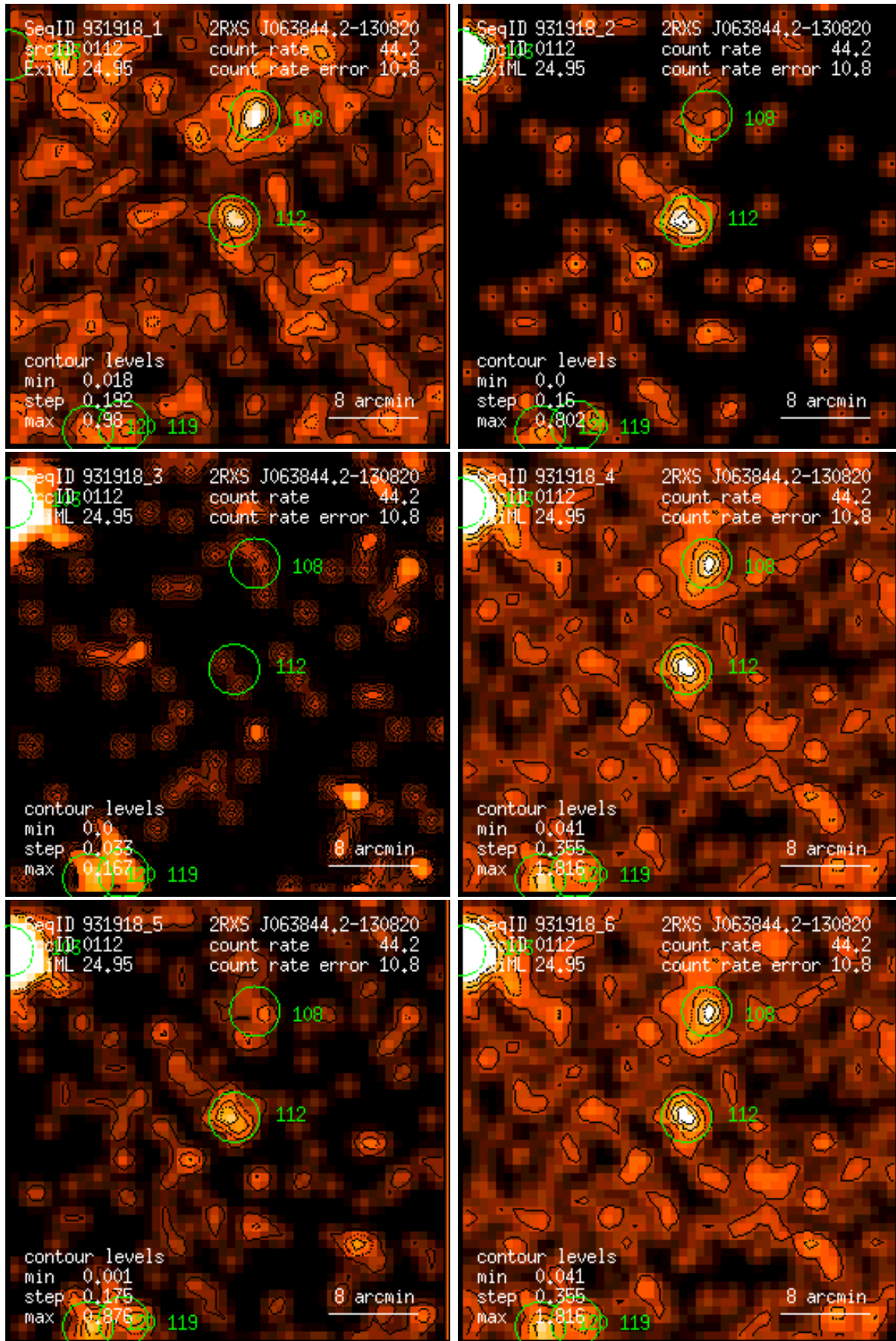
Figure 112: RASS 931918: detection 0112: band rate images, Gaussian filter: (1) PSPC channels 11 – 41, (2) 52 – 90, (3) 91 – 201, (4) 11 – 235, (5) 52 – 201, (6) 11 – 201. Broad band rates in counts/ks. Band rate contour levels in counts/ks/arcmin 2 .
