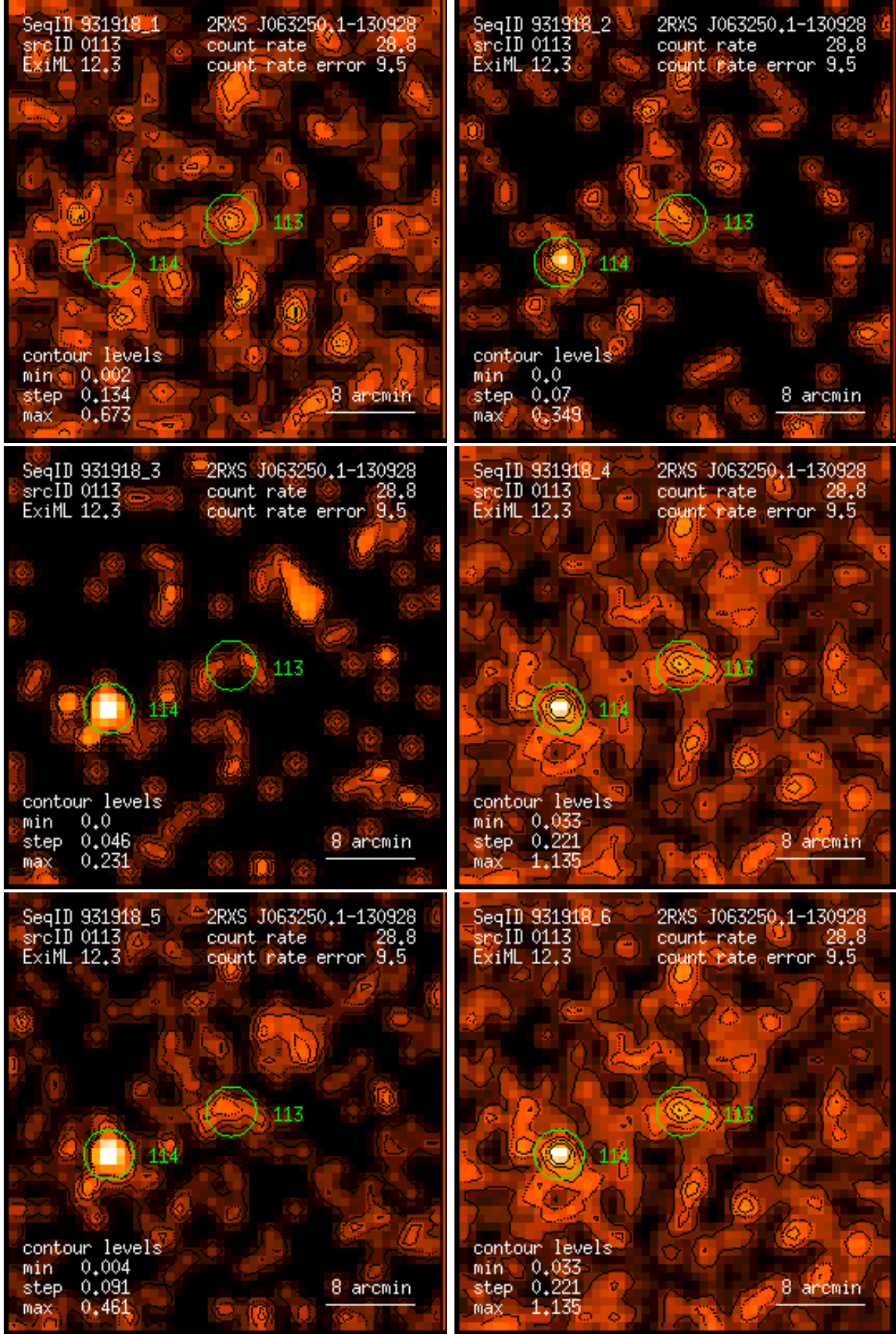
Figure 113: RASS 931918: detection 0113: band rate images, Gaussian filter: (1) PSPC channels 11 – 41, (2) 52 – 90, (3) 91 – 201, (4) 11 – 235, (5) 52 – 201, (6) 11 – 201. Broad band rates in counts/ks. Band rate contour levels in counts/ks/arcmin 2 .
