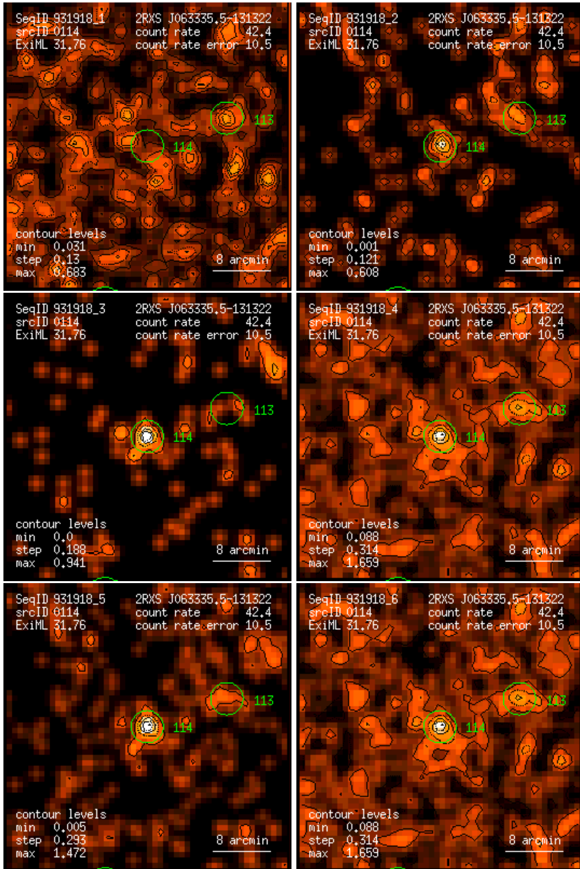
Figure 114: RASS 931918: detection 0114: band rate images, Gaussian filter: (1) PSPC channels 11 – 41, (2) 52 – 90, (3) 91 – 201, (4) 11 – 235, (5) 52 – 201, (6) 11 – 201. Broad band rates in counts/ks. Band rate contour levels in counts/ks/arcmin 2 .
