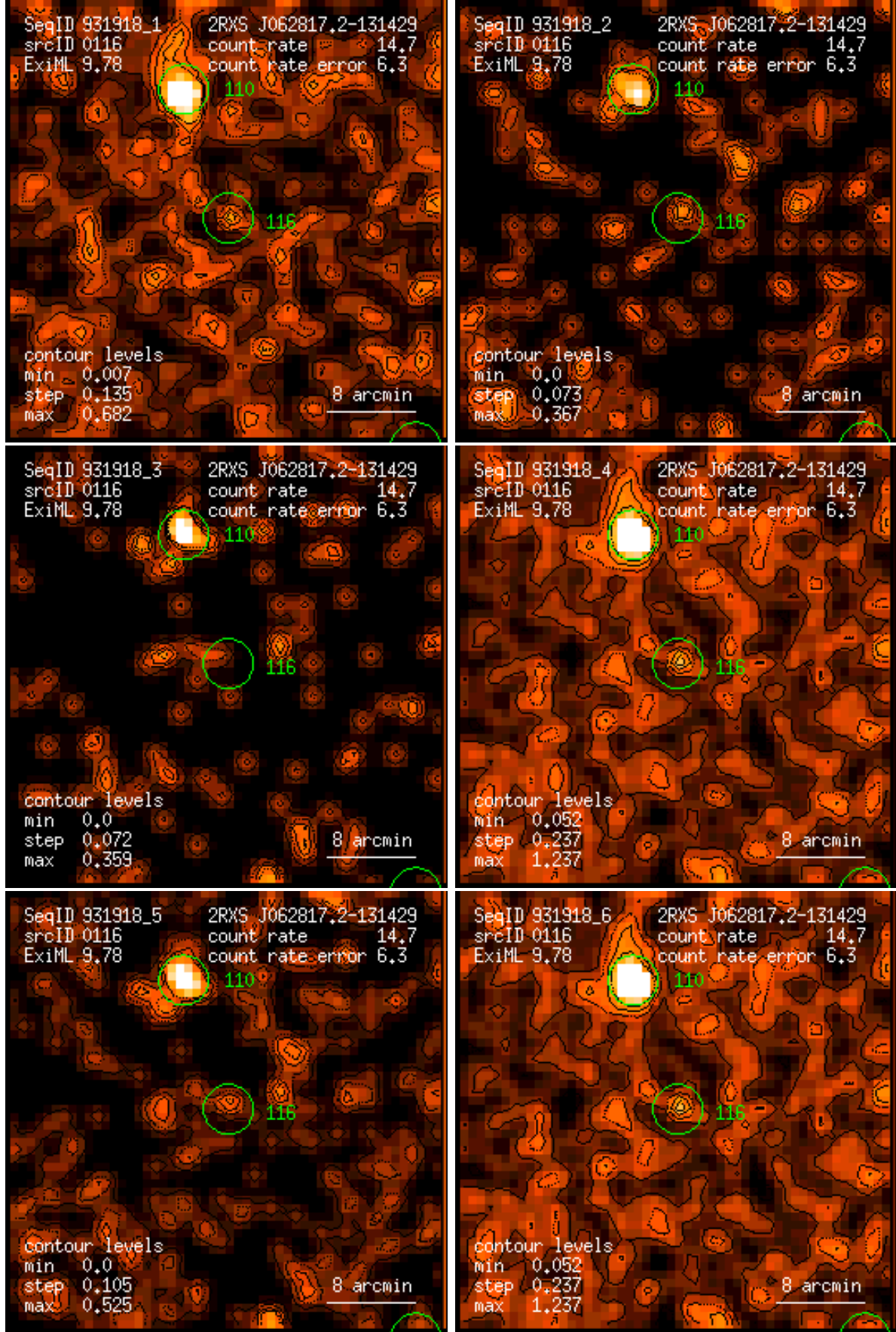
Figure 116: RASS 931918: detection 0116: band rate images, Gaussian filter: (1) PSPC channels 11 – 41, (2) 52 – 90, (3) 91 – 201, (4) 11 – 235, (5) 52 – 201, (6) 11 – 201. Broad band rates in counts/ks. Band rate contour levels in counts/ks/arcmin 2 .
