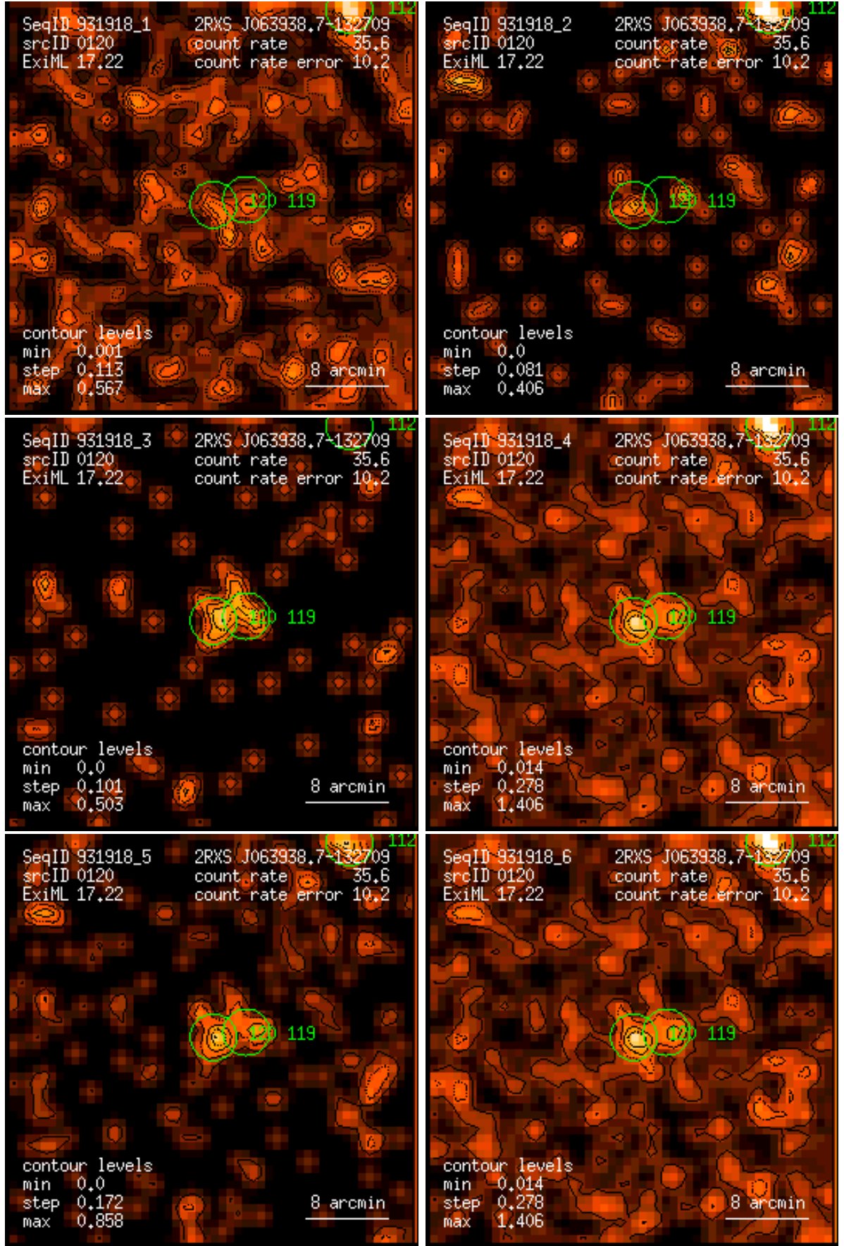
Figure 120: RASS 931918: detection 0120: band rate images, Gaussian filter: (1) PSPC channels 11 – 41, (2) 52 – 90, (3) 91 – 201, (4) 11 – 235, (5) 52 – 201, (6) 11 – 201. Broad band rates in counts/ks. Band rate contour levels in counts/ks/arcmin 2 .
