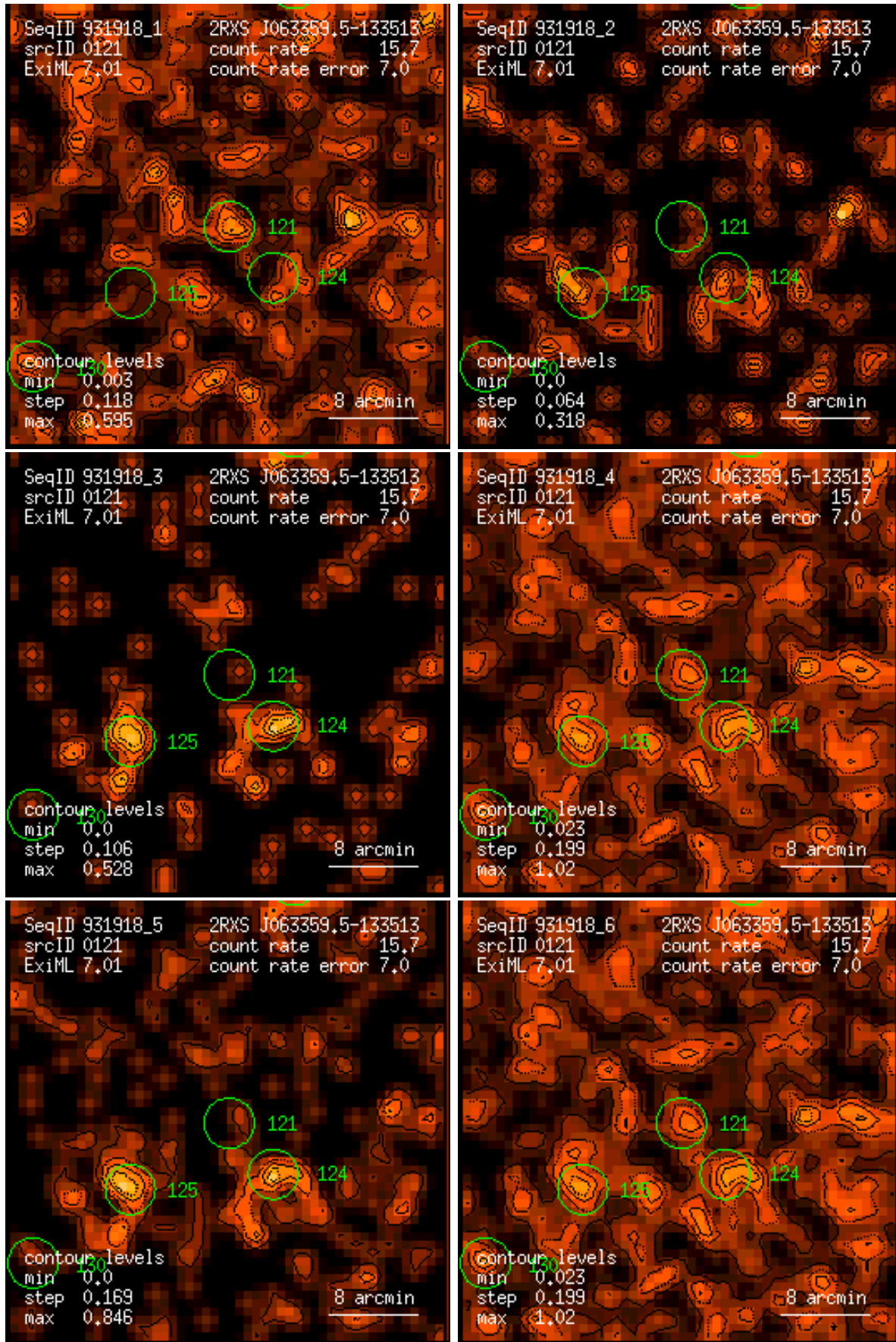
Figure 121: RASS 931918: detection 0121: band rate images, Gaussian filter: (1) PSPC channels 11 – 41, (2) 52 – 90, (3) 91 – 201, (4) 11 – 235, (5) 52 – 201, (6) 11 – 201. Broad band rates in counts/ks. Band rate contour levels in counts/ks/arcmin 2 .
