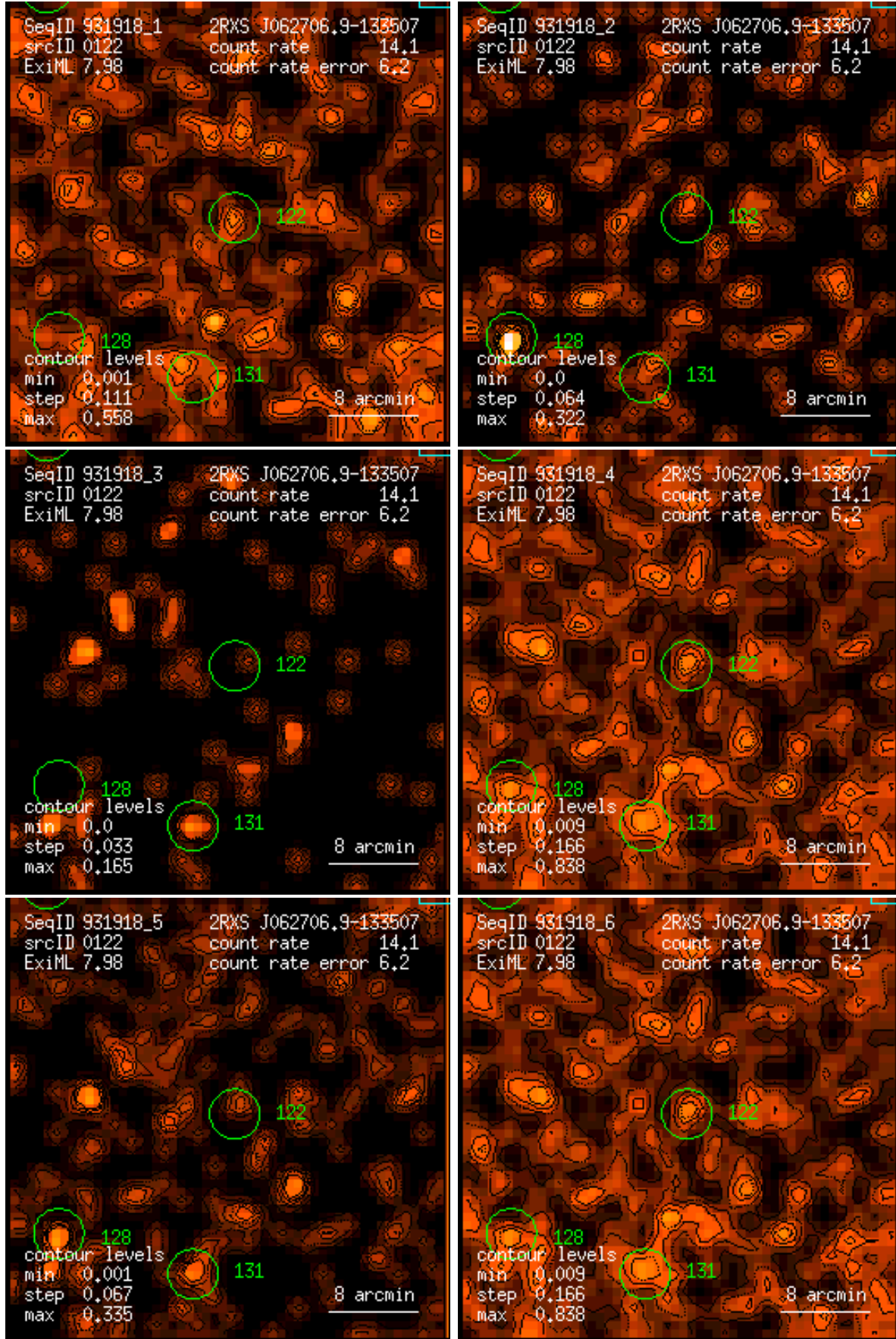
Figure 122: RASS 931918: detection 0122: band rate images, Gaussian filter: (1) PSPC channels 11 – 41, (2) 52 – 90, (3) 91 – 201, (4) 11 – 235, (5) 52 – 201, (6) 11 – 201. Broad band rates in counts/ks. Band rate contour levels in counts/ks/arcmin 2 .
