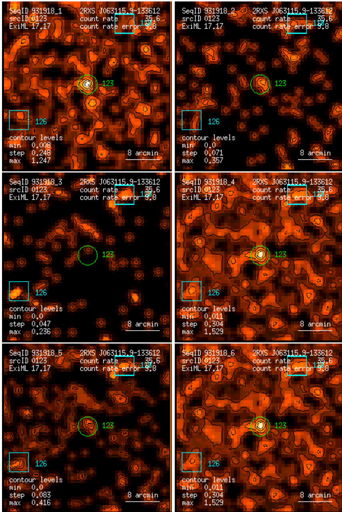
Figure 123: RASS 931918: detection 0123: band rate images, Gaussian filter: (1) PSPC channels 11 – 41, (2) 52 – 90, (3) 91 – 201, (4) 11 – 235, (5) 52 – 201, (6) 11 – 201. Broad band rates in counts/ks. Band rate contour levels in counts/ks/arcmin 2 .
