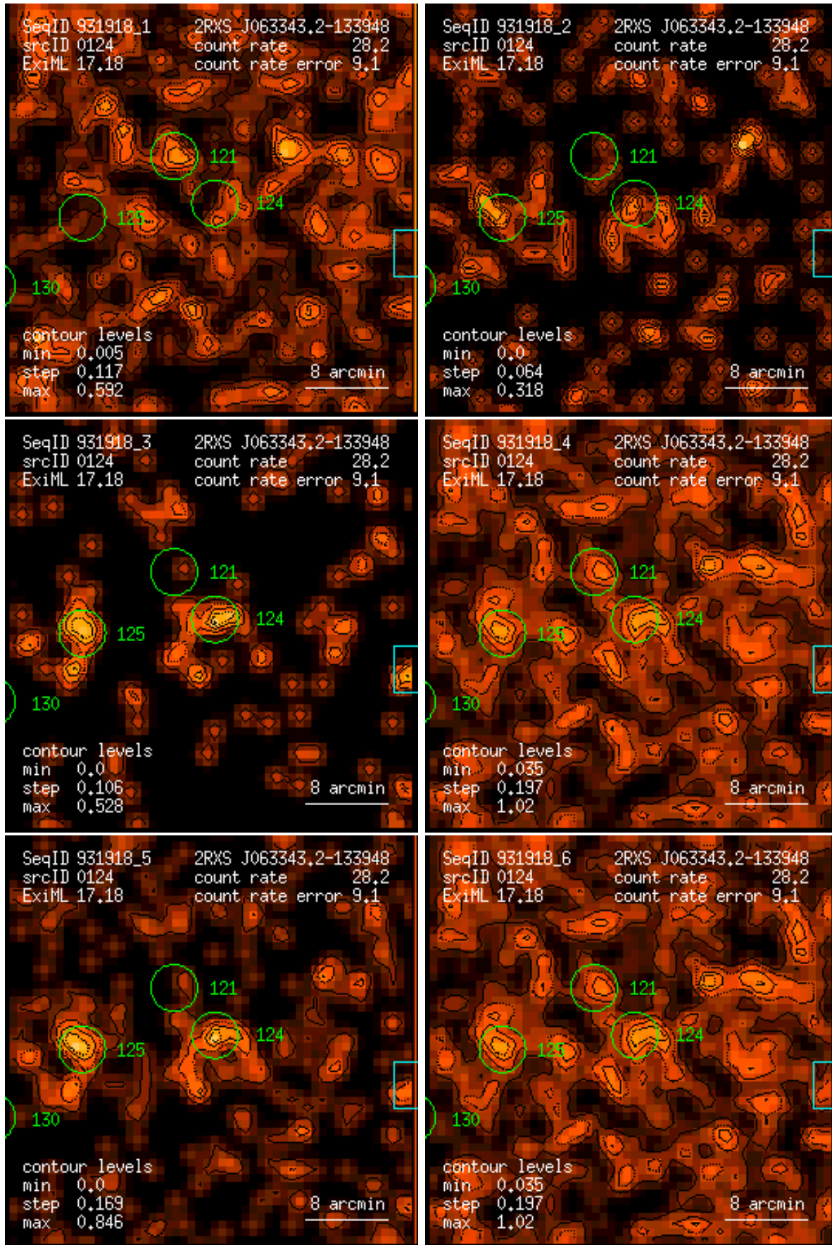
Figure 124: RASS 931918: detection 0124: band rate images, Gaussian filter: (1) PSPC channels 11 – 41, (2) 52 – 90, (3) 91 – 201, (4) 11 – 235, (5) 52 – 201, (6) 11 – 201. Broad band rates in counts/ks. Band rate contour levels in counts/ks/arcmin 2 .
