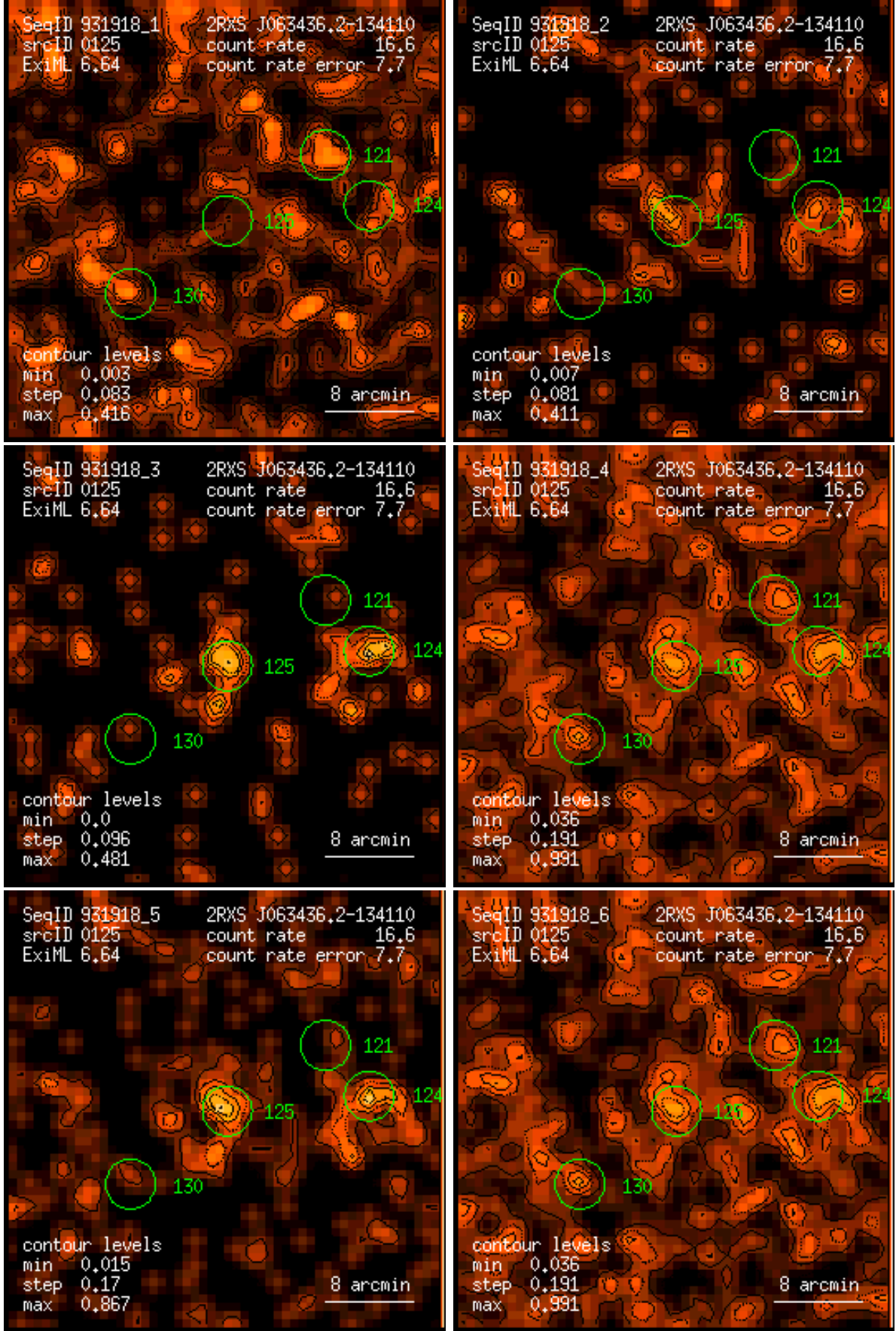
Figure 125: RASS 931918: detection 0125: band rate images, Gaussian filter: (1) PSPC channels 11 – 41, (2) 52 – 90, (3) 91 – 201, (4) 11 – 235, (5) 52 – 201, (6) 11 – 201. Broad band rates in counts/ks. Band rate contour levels in counts/ks/arcmin 2 .
