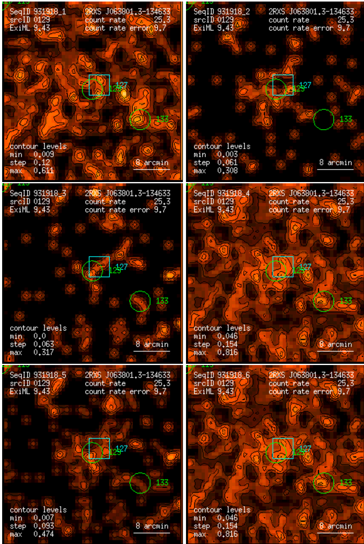
Figure 129: RASS 931918: detection 0129: band rate images, Gaussian filter: (1) PSPC channels 11 – 41, (2) 52 – 90, (3) 91 – 201, (4) 11 – 235, (5) 52 – 201, (6) 11 – 201. Broad band rates in counts/ks. Band rate contour levels in counts/ks/arcmin 2 .
