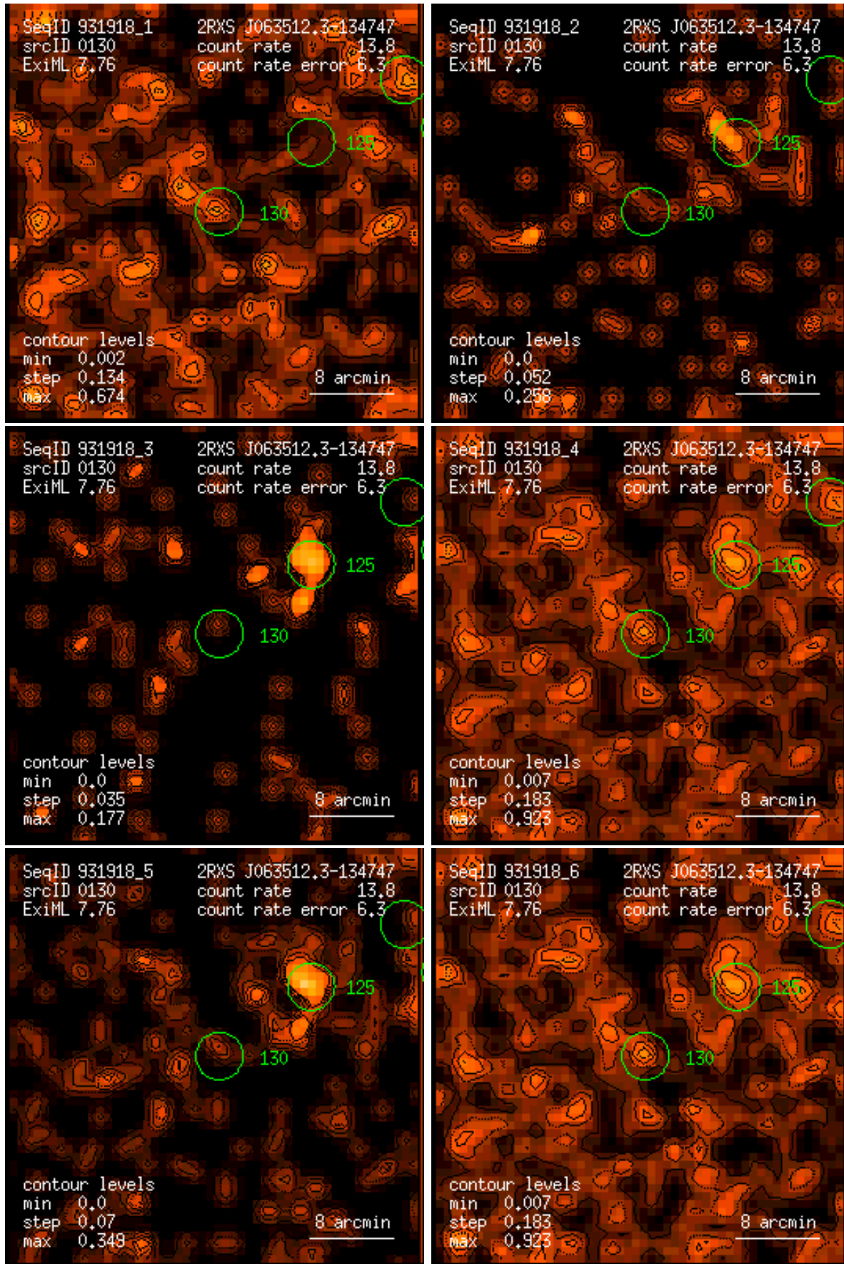
Figure 130: RASS 931918: detection 0130: band rate images, Gaussian filter: (1) PSPC channels 11 – 41, (2) 52 – 90, (3) 91 – 201, (4) 11 – 235, (5) 52 – 201, (6) 11 – 201. Broad band rates in counts/ks. Band rate contour levels in counts/ks/arcmin 2 .
