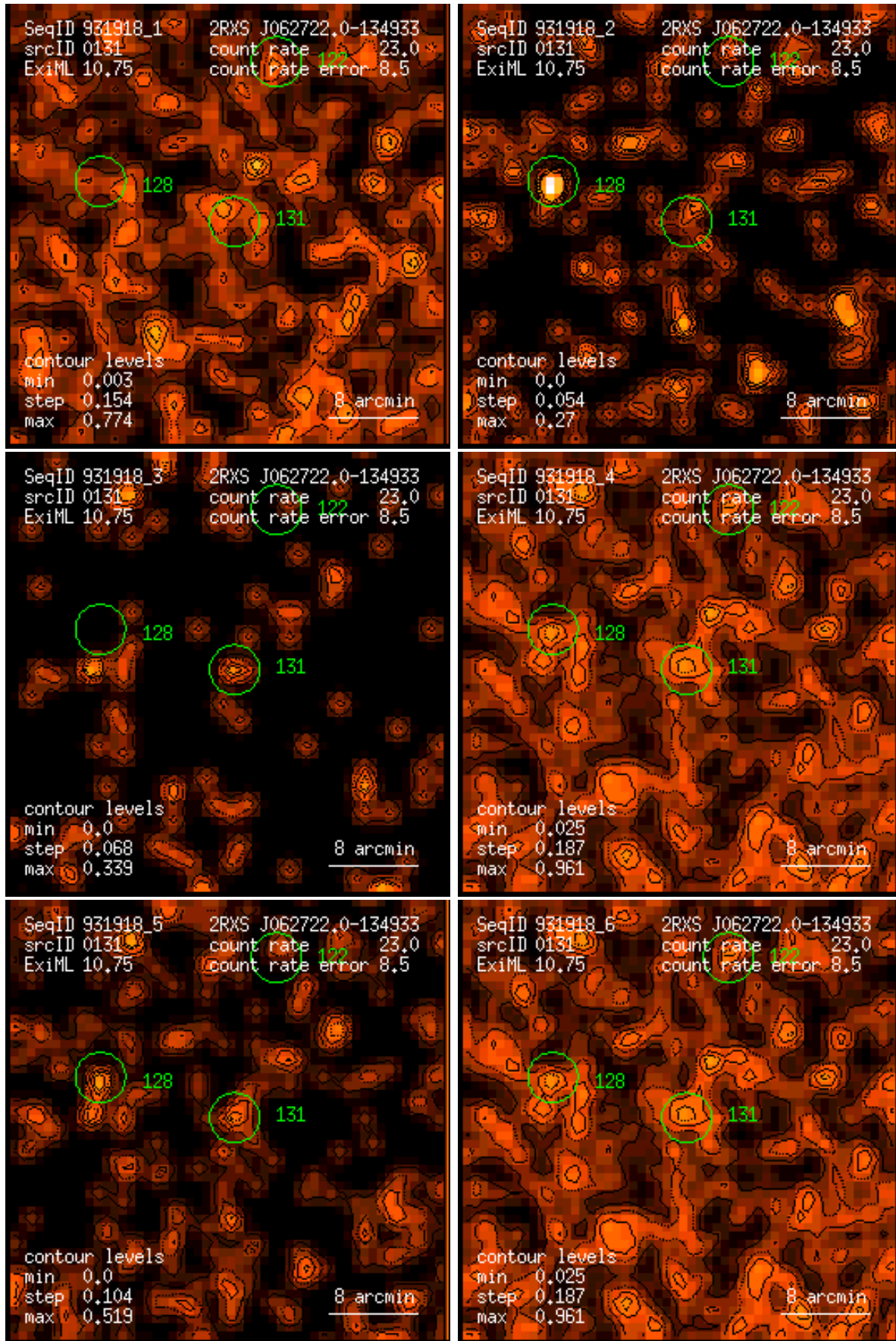
Figure 131: RASS 931918: detection 0131: band rate images, Gaussian filter: (1) PSPC channels 11 – 41, (2) 52 – 90, (3) 91 – 201, (4) 11 – 235, (5) 52 – 201, (6) 11 – 201. Broad band rates in counts/ks. Band rate contour levels in counts/ks/arcmin 2 .
