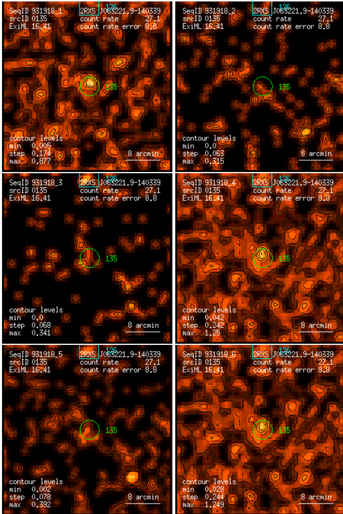
Figure 135: RASS 931918: detection 0135: band rate images, Gaussian filter: (1) PSPC channels 11 – 41, (2) 52 – 90, (3) 91 – 201, (4) 11 – 235, (5) 52 – 201, (6) 11 – 201. Broad band rates in counts/ks. Band rate contour levels in counts/ks/arcmin 2 .
