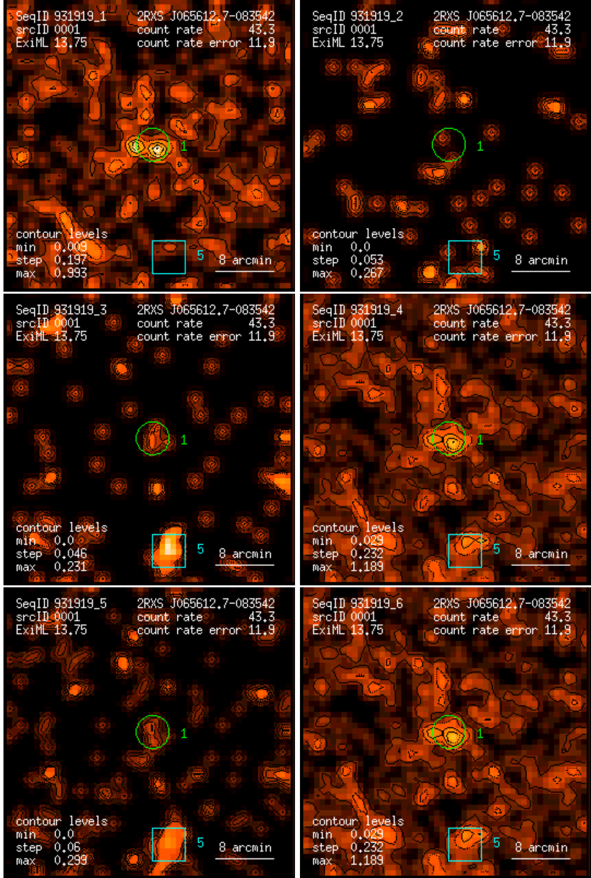
Figure 1: RASS 931919: detection 0001: band rate images, Gaussian filter: (1) PSPC channels 11 – 41, (2) 52 – 90, (3) 91 – 201, (4) 11 – 235, (5) 52 – 201, (6) 11 – 201. Broad band rates in counts/ks. Band rate contour levels in counts/ks/arcmin 2 .
