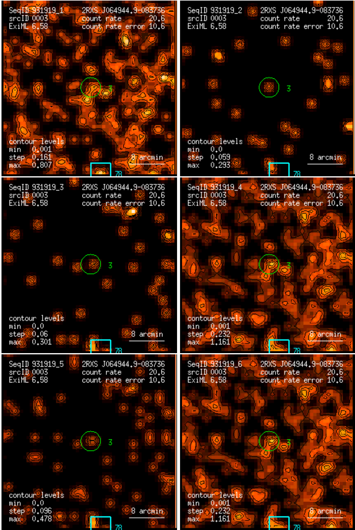
Figure 3: RASS 931919: detection 0003: band rate images, Gaussian filter: (1) PSPC channels 11 – 41, (2) 52 – 90, (3) 91 – 201, (4) 11 – 235, (5) 52 – 201, (6) 11 – 201. Broad band rates in counts/ks. Band rate contour levels in counts/ks/arcmin 2 .
