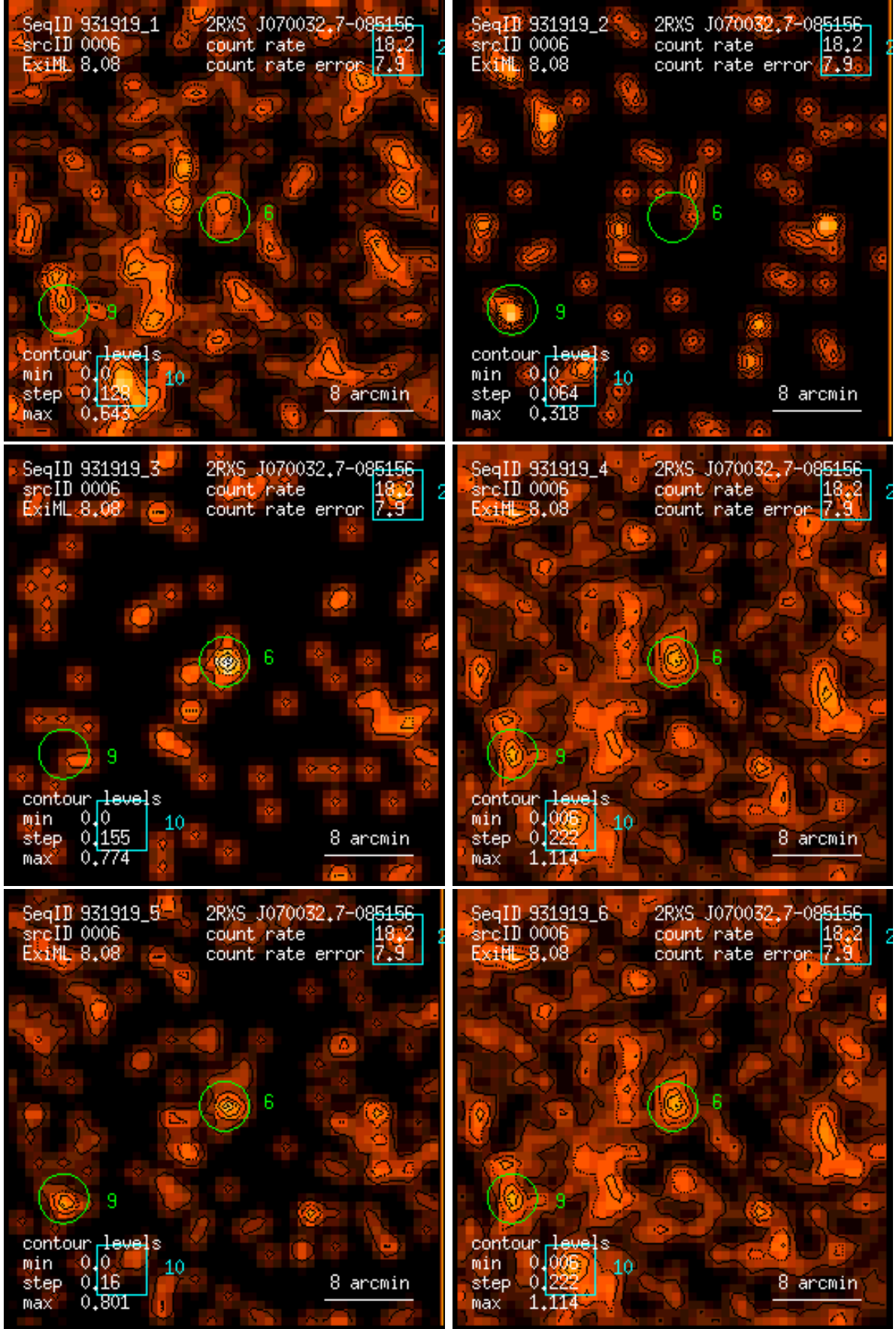
Figure 6: RASS 931919: detection 0006: band rate images, Gaussian filter: (1) PSPC channels 11 – 41, (2) 52 – 90, (3) 91 – 201, (4) 11 – 235, (5) 52 – 201, (6) 11 – 201. Broad band rates in counts/ks. Band rate contour levels in counts/ks/arcmin 2 .
