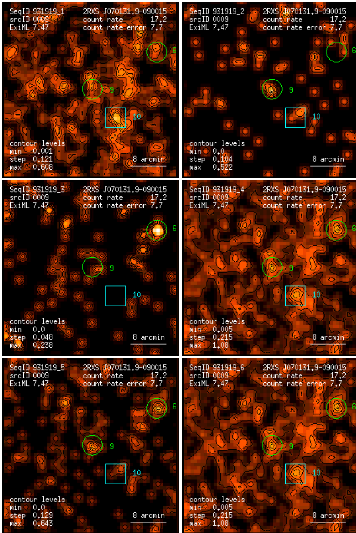
Figure 9: RASS 931919: detection 0009: band rate images, Gaussian filter: (1) PSPC channels 11 – 41, (2) 52 – 90, (3) 91 – 201, (4) 11 – 235, (5) 52 – 201, (6) 11 – 201. Broad band rates in counts/ks. Band rate contour levels in counts/ks/arcmin 2 .
