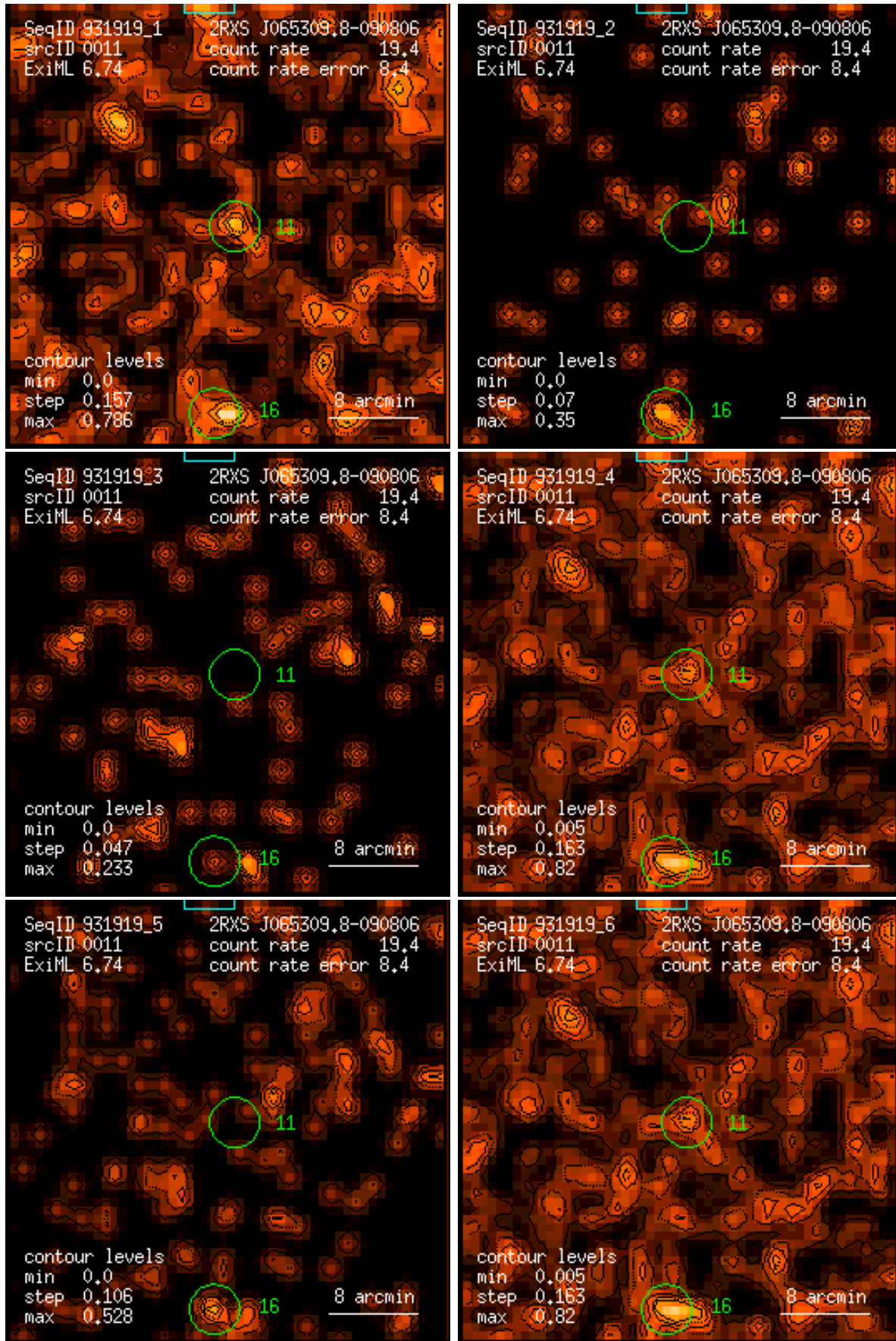
Figure 11: RASS 931919: detection 0011: band rate images, Gaussian filter: (1) PSPC channels 11 – 41, (2) 52 – 90, (3) 91 – 201, (4) 11 – 235, (5) 52 – 201, (6) 11 – 201. Broad band rates in counts/ks. Band rate contour levels in counts/ks/arcmin 2 .
