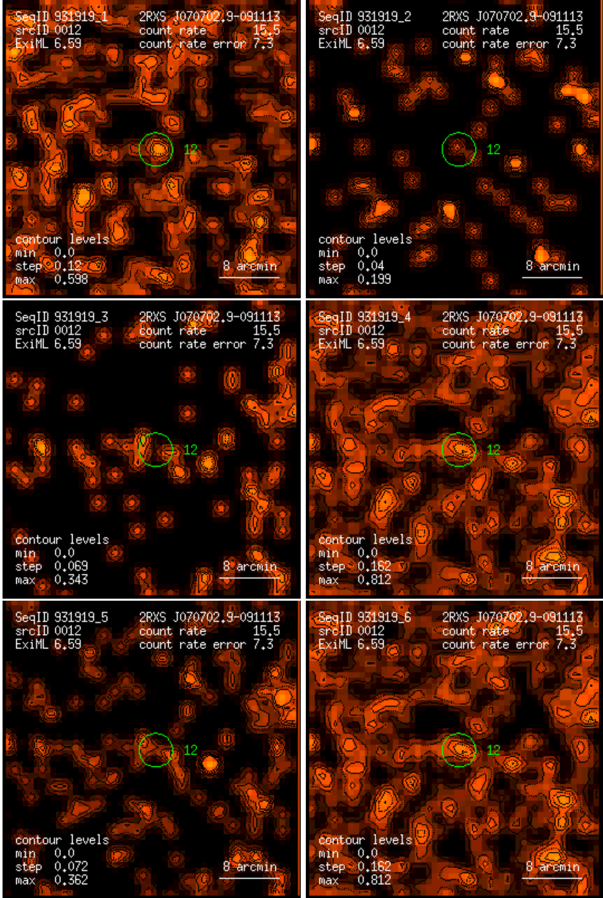
Figure 12: RASS 931919: detection 0012: band rate images, Gaussian filter: (1) PSPC channels 11 – 41, (2) 52 – 90, (3) 91 – 201, (4) 11 – 235, (5) 52 – 201, (6) 11 – 201. Broad band rates in counts/ks. Band rate contour levels in counts/ks/arcmin 2 .
