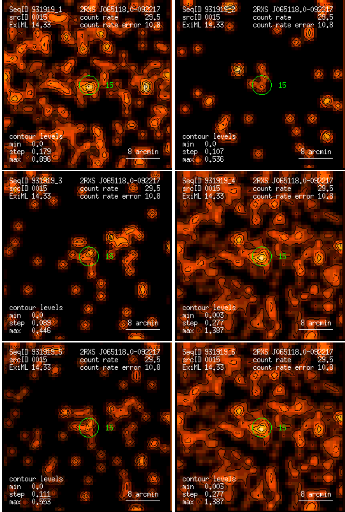
Figure 15: RASS 931919: detection 0015: band rate images, Gaussian filter: (1) PSPC channels 11 – 41, (2) 52 – 90, (3) 91 – 201, (4) 11 – 235, (5) 52 – 201, (6) 11 – 201. Broad band rates in counts/ks. Band rate contour levels in counts/ks/arcmin 2 .
